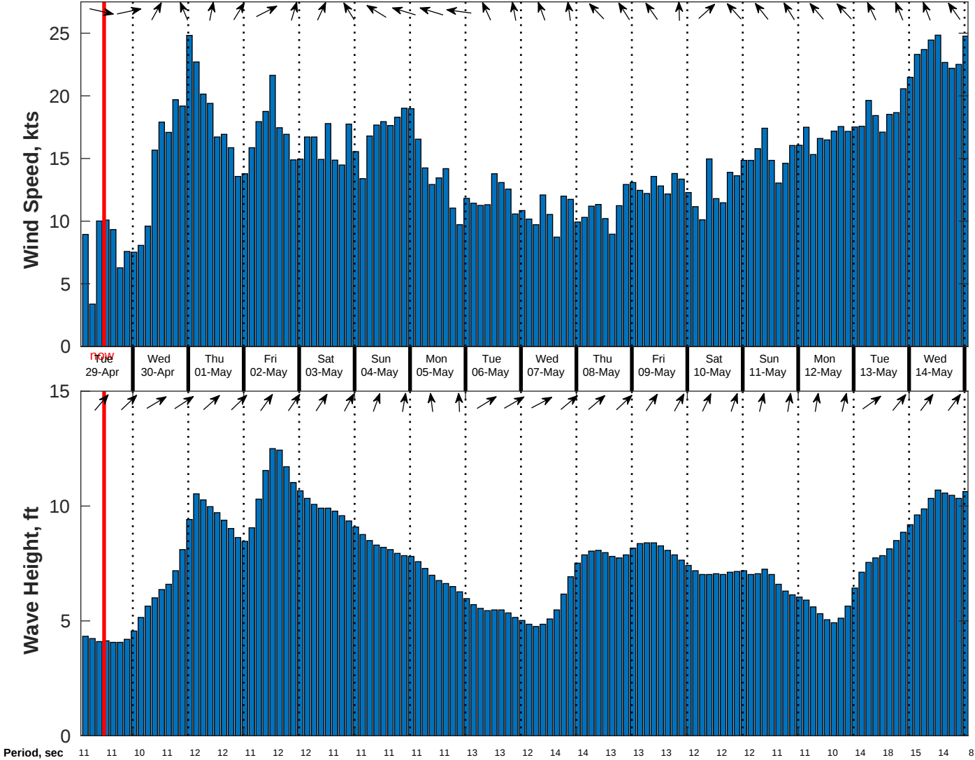
Wind & Wave Forecast for Benthic Solutions South Africa HF Site2 from 28-Apr-2025 02:00:00 to 14-May-2025 02:00:00
