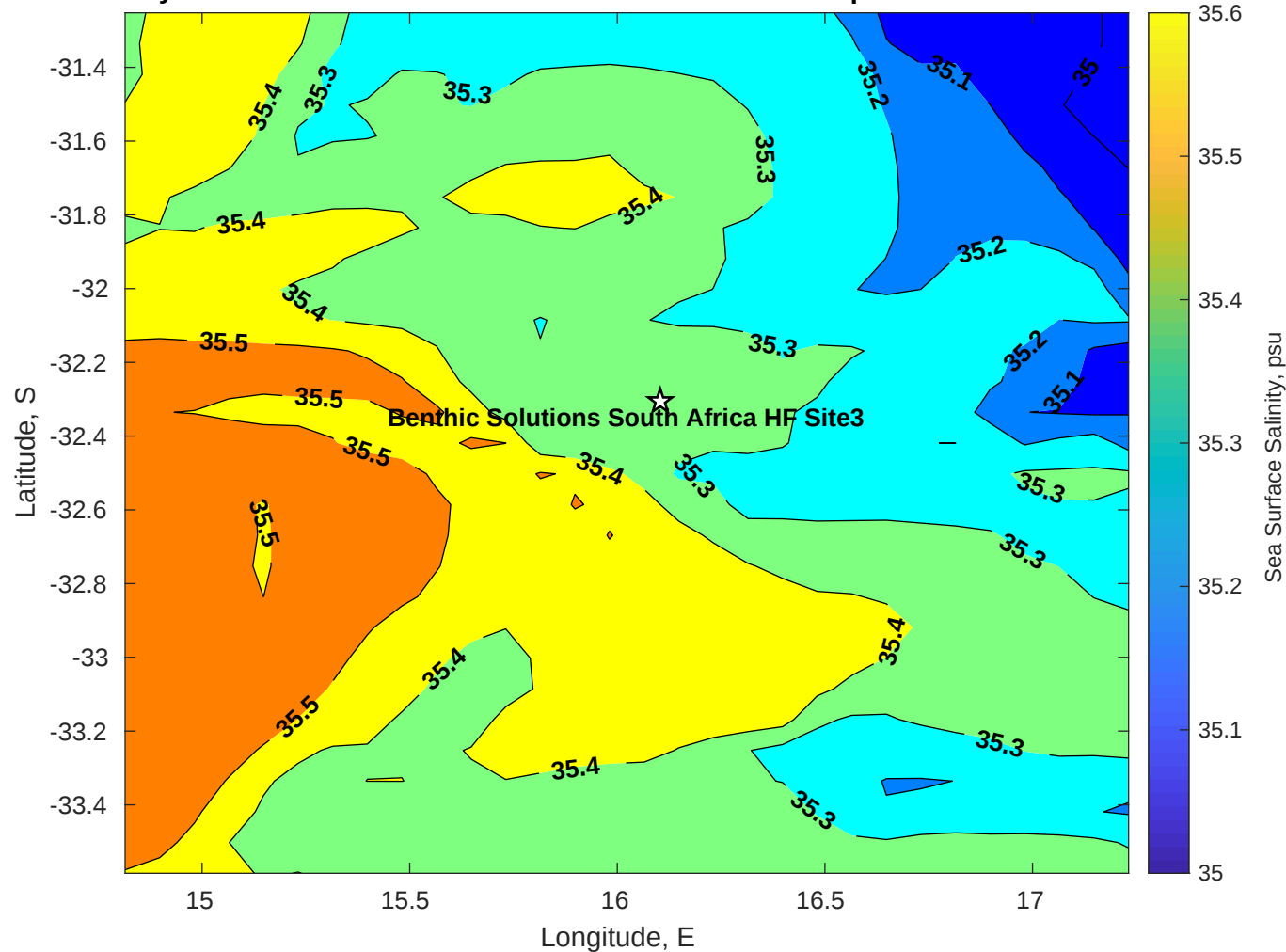
Surface Salinity for Benthic Solutions South Africa HF Site3 at 27-Apr-2025 00:00:00
