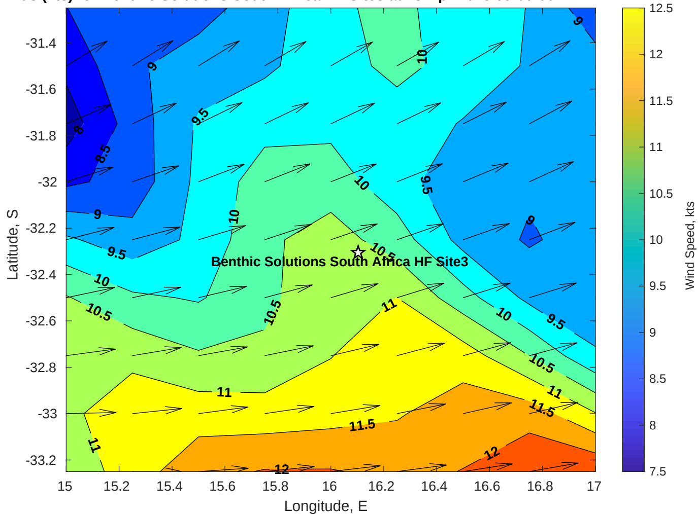
Winds (kts) for Benthic Solutions South Africa HF Site3 at 28-Apr-2025 09:00:00
