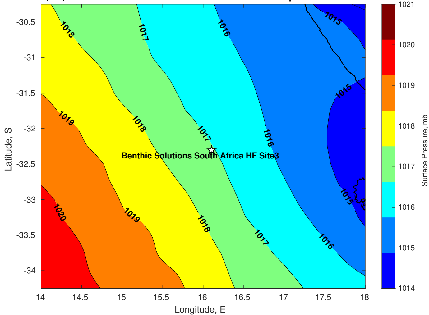
Surface Pressure (mb) for Benthic Solutions South Africa HF Site3 at 30-Apr-2025 00:00:00
