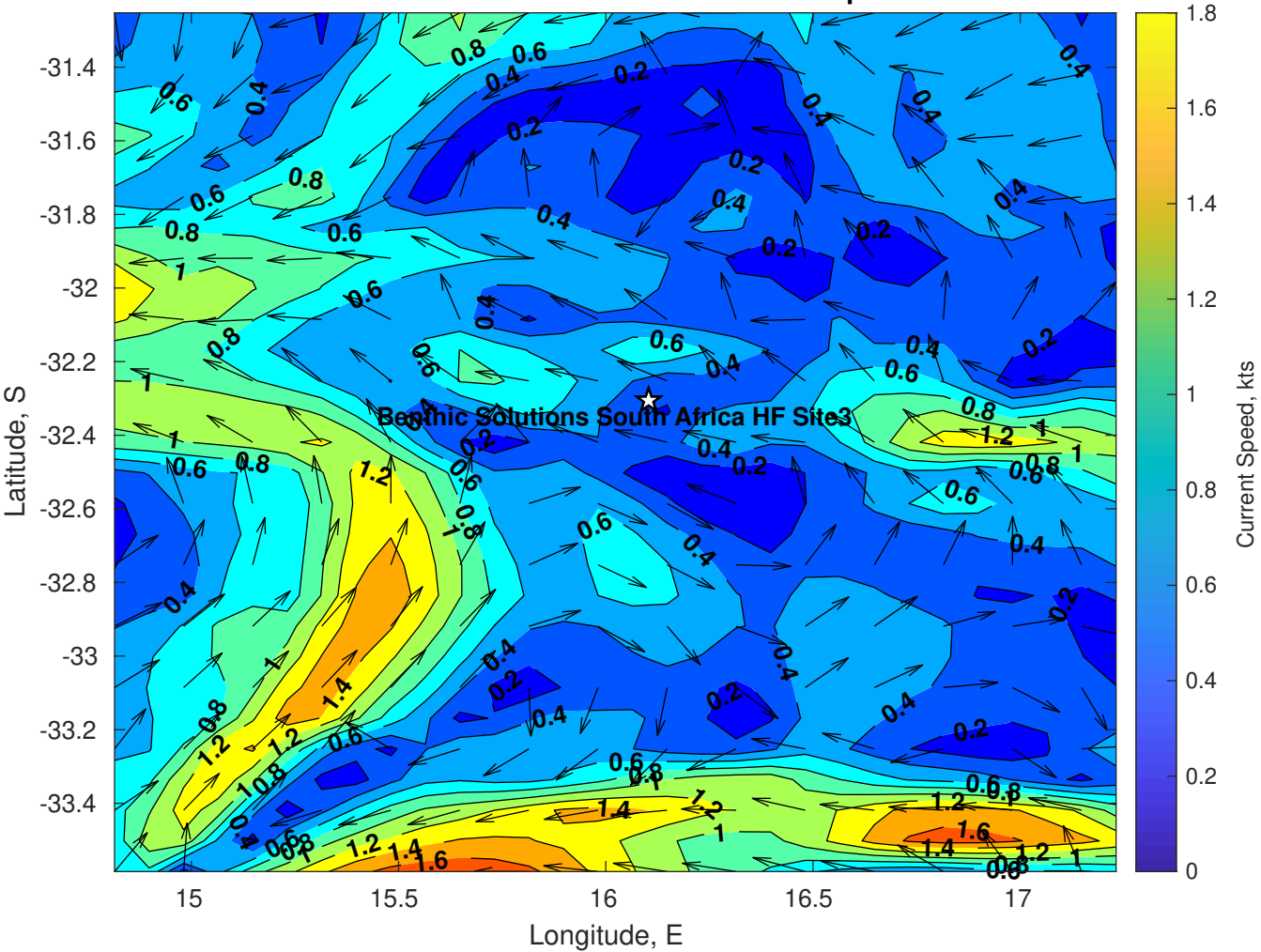
Surface Currents for Benthic Solutions South Africa HF Site3 at 27-Apr-2025 00:00:00
