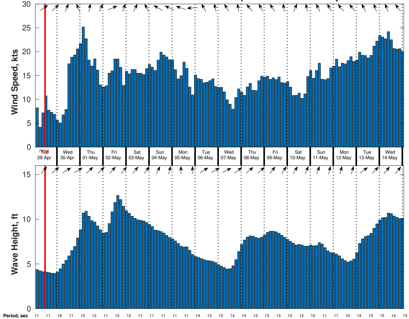
Wind & Wave Forecast for Benthic Solutions South Africa HF Site3 from 28-Apr-2025 02:00:00 to 14-May-2025 02:00:00
