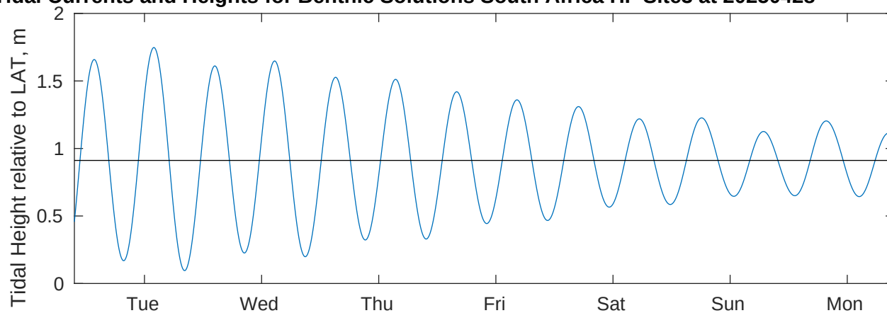
Tidal Currents and Heights for Benthic Solutions South Africa HF Site3 at 20250428
