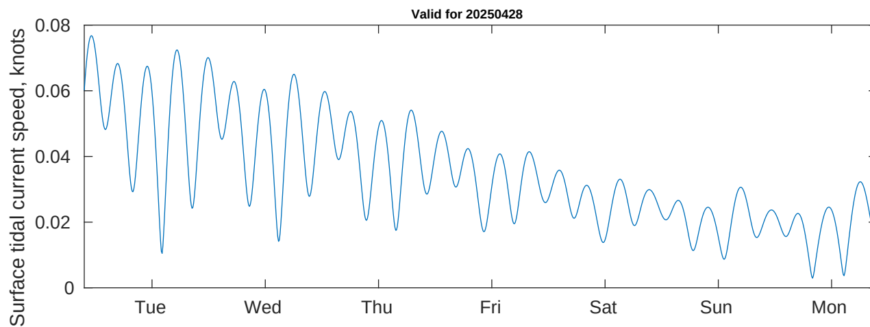
Tidal Currents and Heights for Benthic Solutions South Africa HF Site3 at 20250428
