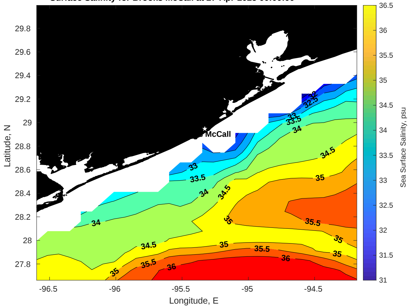
Surface Salinity for Brooks McCall at 27-Apr-2025 00:00:00
