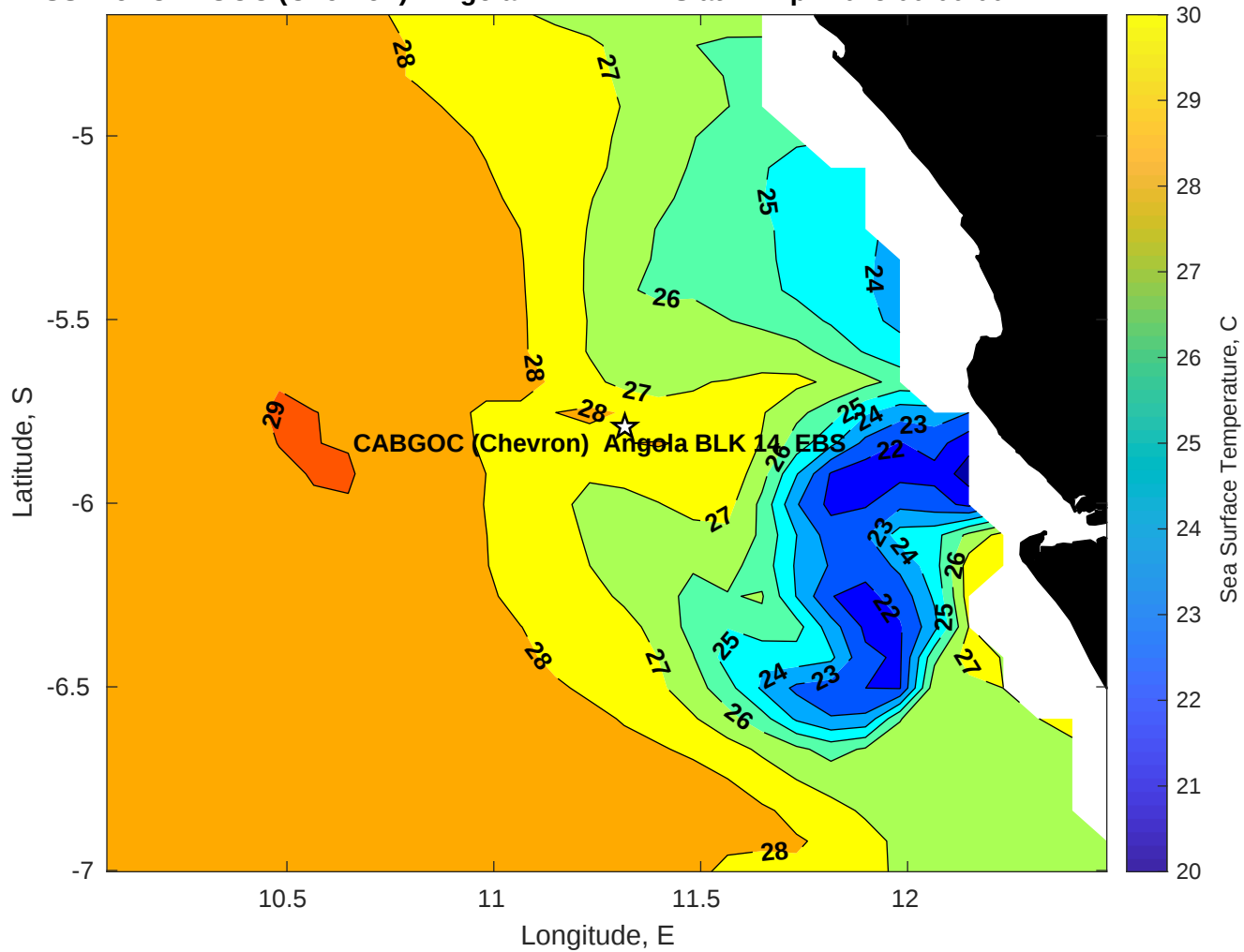
SST for CABGOC (Chevron) Angola BLK 14 EBS at 27-Apr-2025 00:00:00
