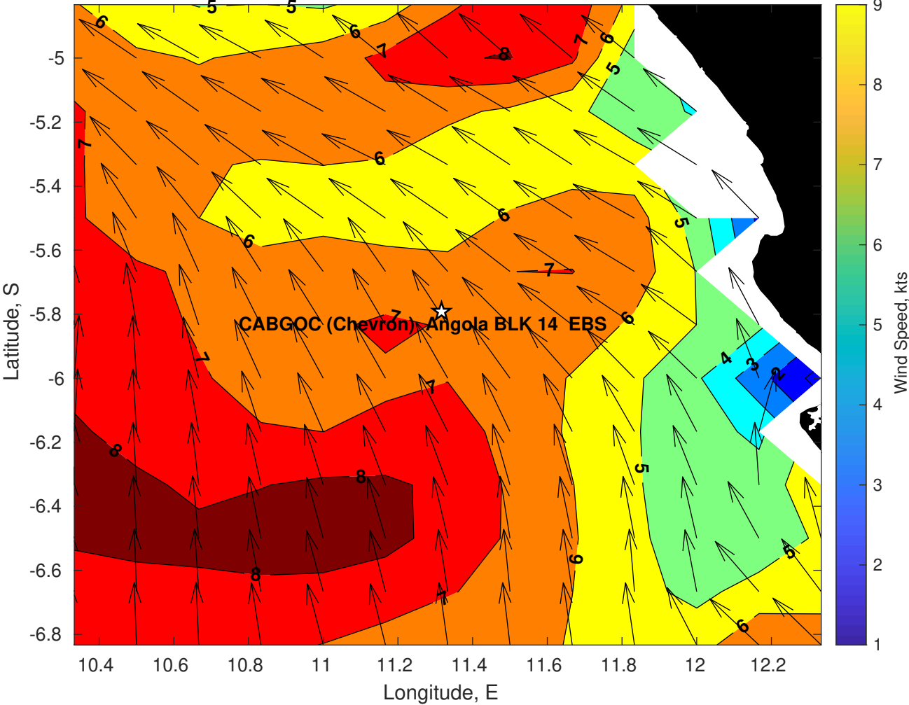
Winds (kts) for CABGOC (Chevron) Angola BLK 14 EBS at 28-Apr-2025 09:00:00
