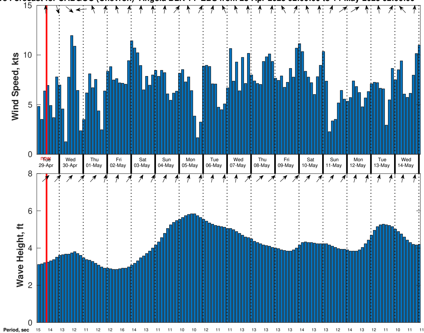
Wind & Wave Forecast for CABGOC (Chevron) Angola BLK 14 EBS from 28-Apr-2025 02:00:00 to 14-May-2025 02:00:00
