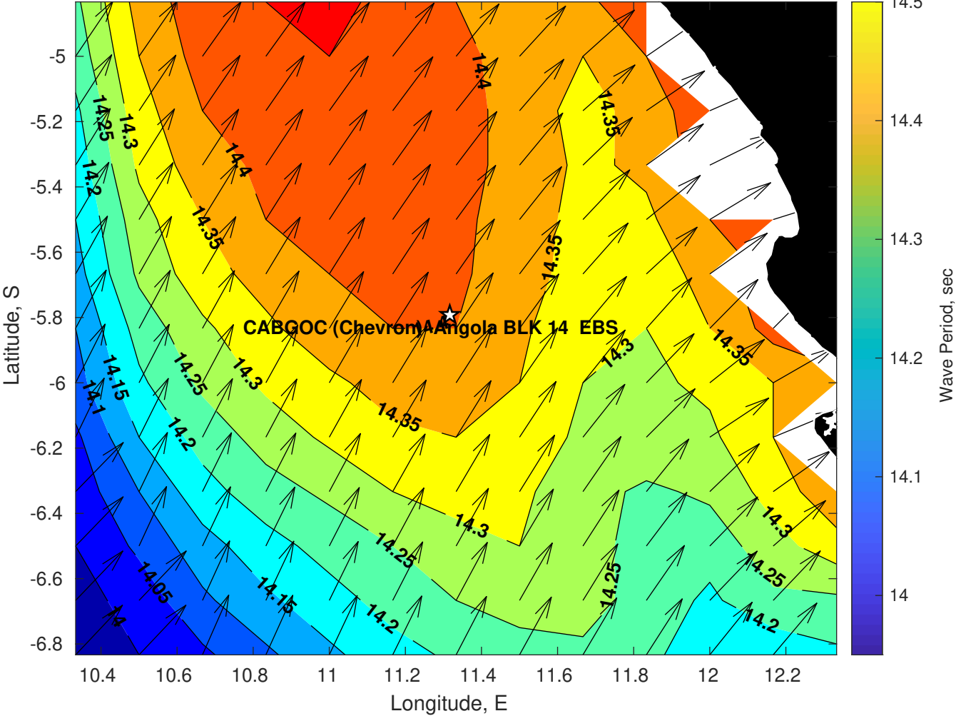
Wave Period (sec) for CABGOC (Chevron) Angola BLK 14 EBS at 28-Apr-2025 09:00:00
