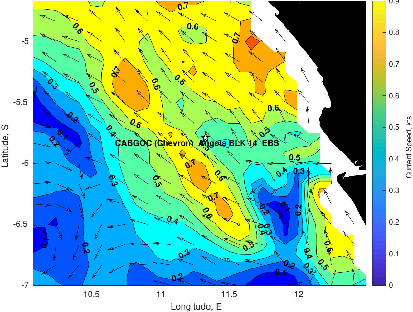
Surface Currents for CABGOC (Chevron) Angola BLK 14 EBS at 27-Apr-2025 00:00:00
