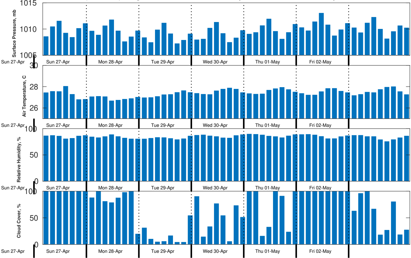
Met Forecast for CABGOC (Chevron) Angola BLK 14 EBS from 28-Apr-2025 00:00:00 to 05-May-2025 00:00:00
