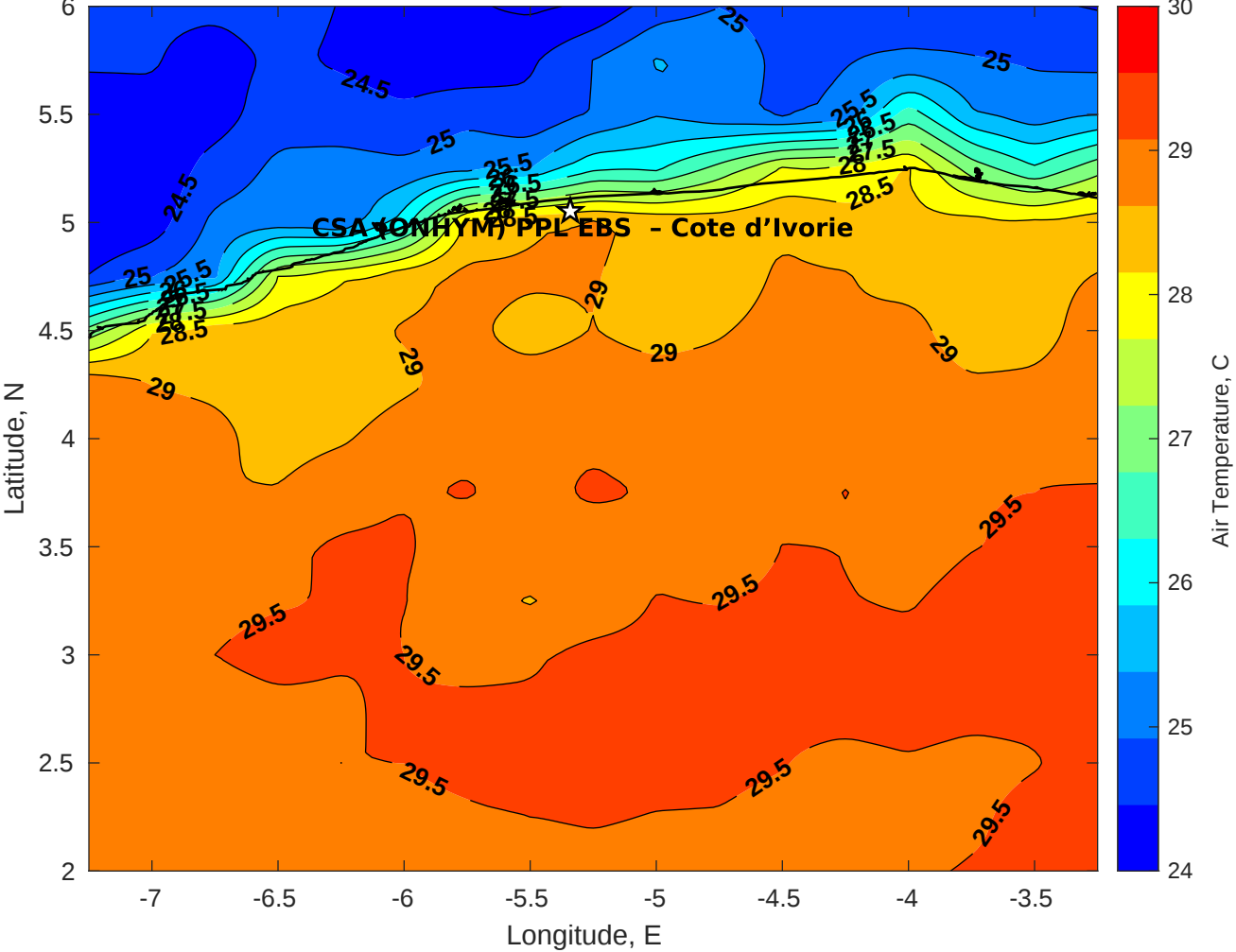
Air Temperature (C) for CSA (ONHYM) PPL EBS - Cote d'Ivoire at 28-Apr-2025
