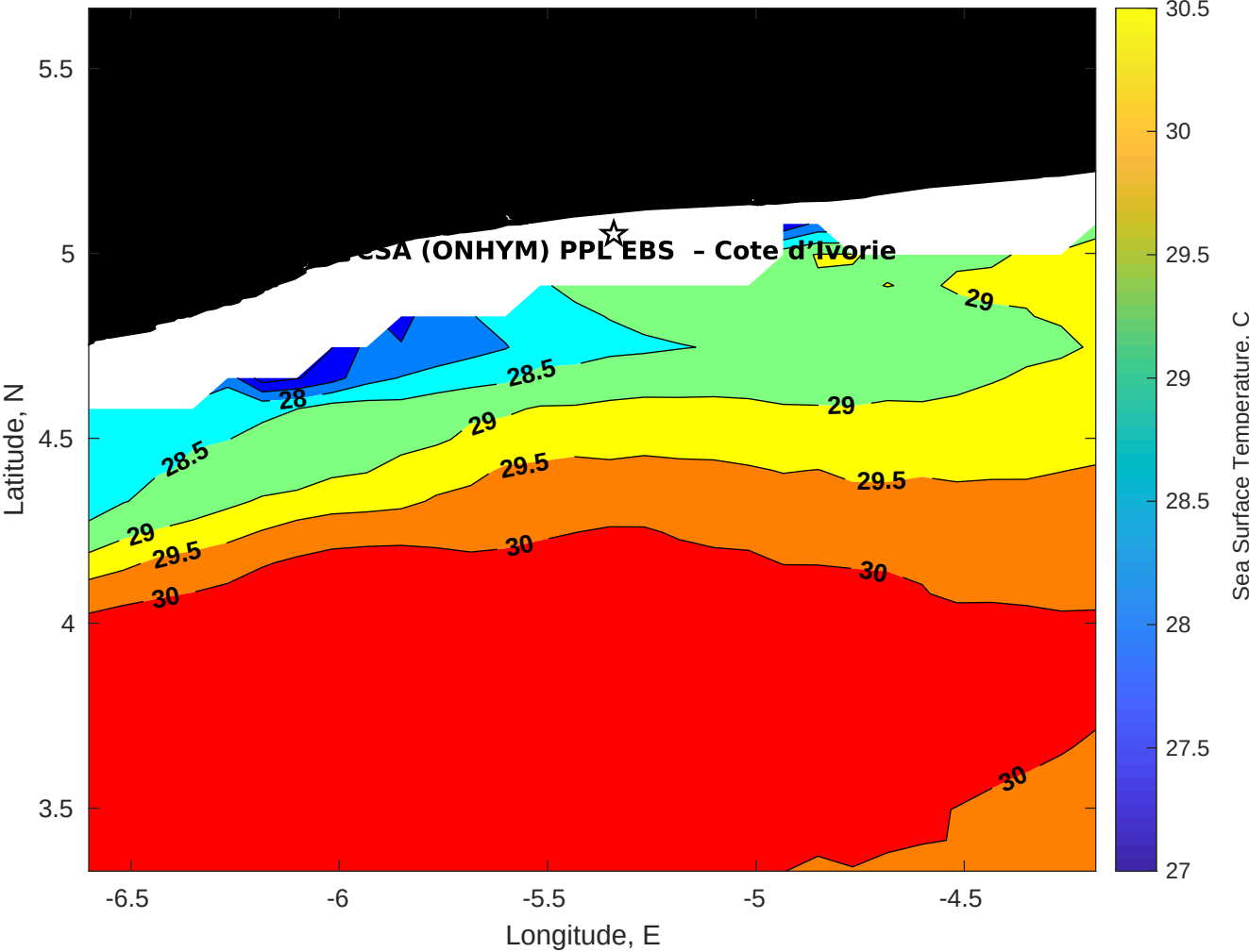
SST for CSA (ONHYM) PPL EBS - Cote d'Ivoire at 27-Apr-2025 00:00:00
