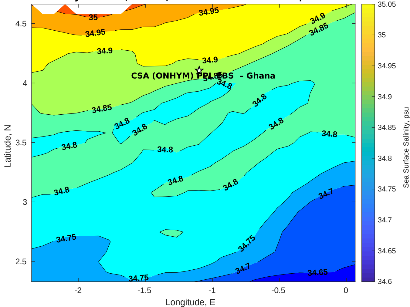
Surface Salinity for CSA (ONHYM) PPL EBS - Ghana at 27-Apr-2025 00:00:00
