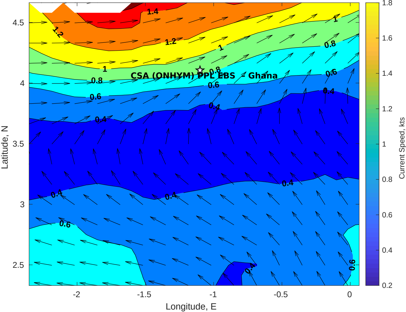
Surface Currents for CSA (ONHYM) PPL EBS - Ghana at 27-Apr-2025 00:00:00
