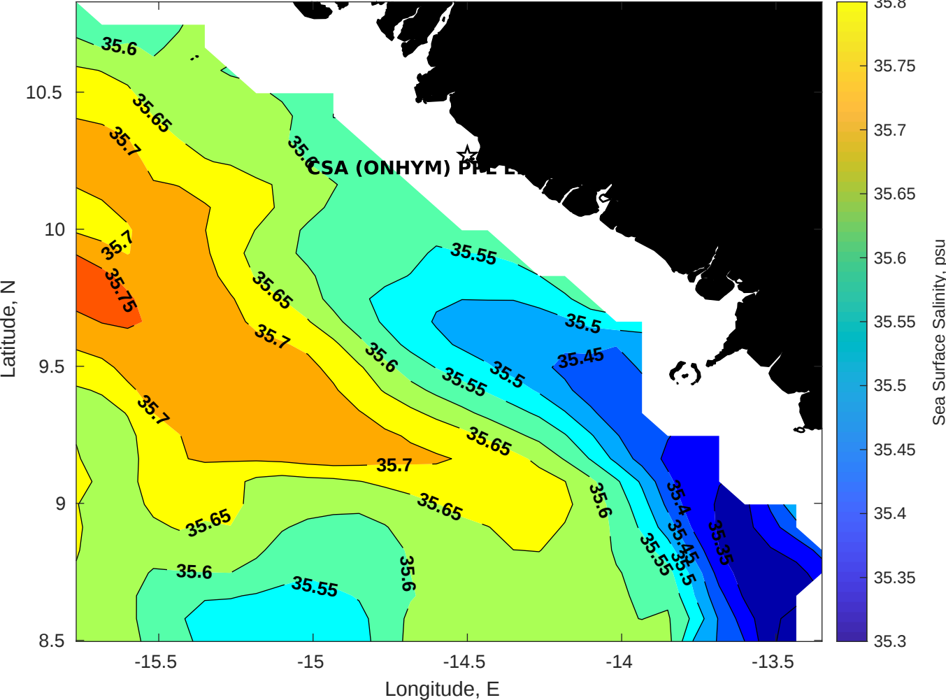
Surface Salinity for CSA (ONHYM) PPL EBS - Guinea at 27-Apr-2025 00:00:00
