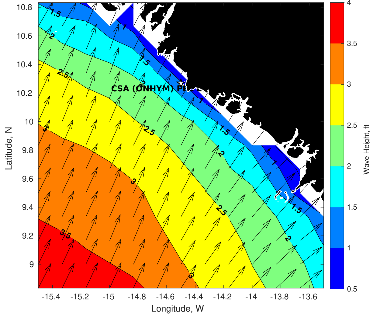
Wave Height (ft) for CSA (ONHYM) PPL EBS - Guinea at 28-Apr-2025 09:00:00
