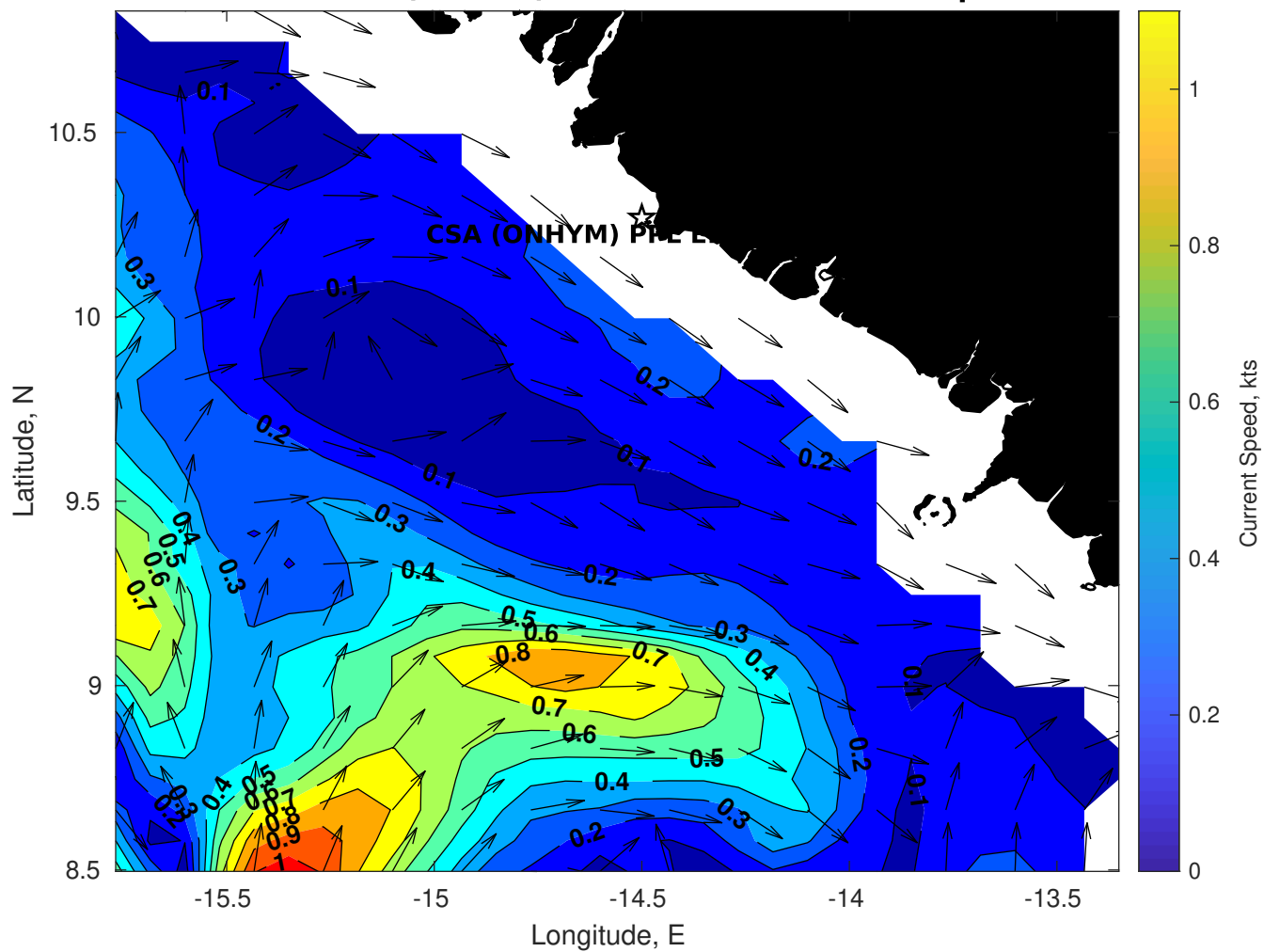
Surface Currents for CSA (ONHYM) PPL EBS - Guinea at 27-Apr-2025 00:00:00
