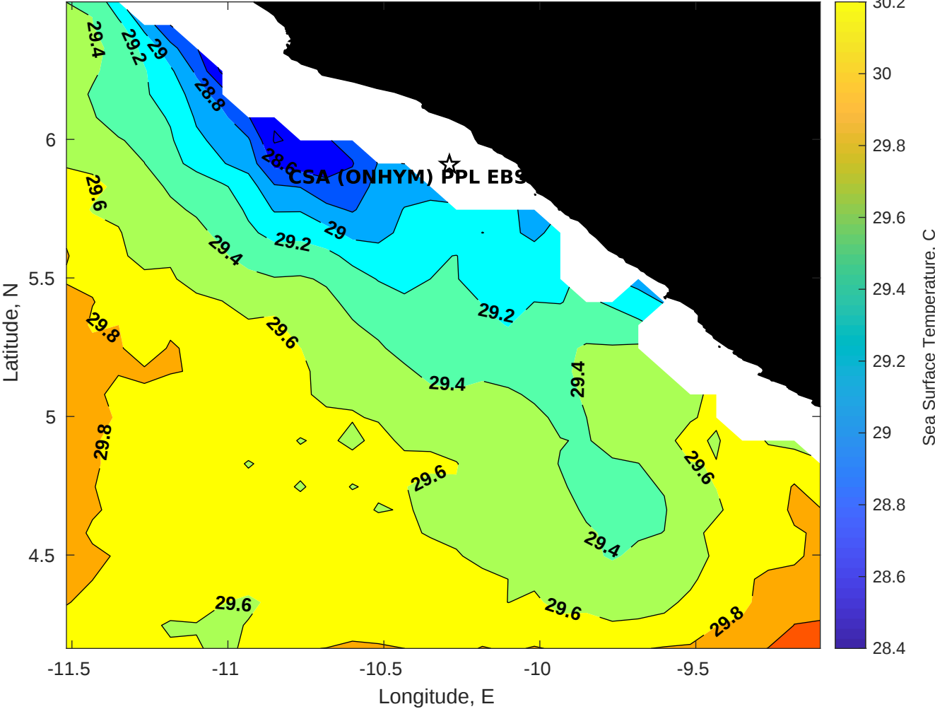
SST for CSA (ONHYM) PPL EBS - Liberia at 27-Apr-2025 00:00:00
