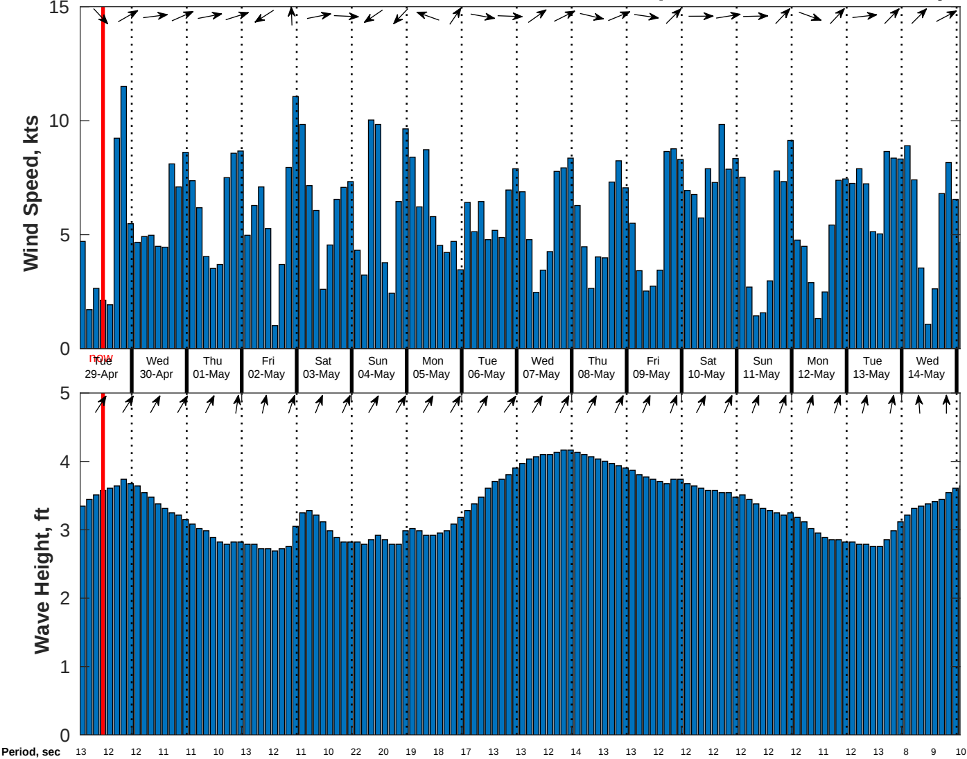
Wind & Wave Forecast for CSA (ONHYM) PPL EBS - Liberia from 28-Apr-2025 01:00:00 to 14-May-2025 01:00:00
