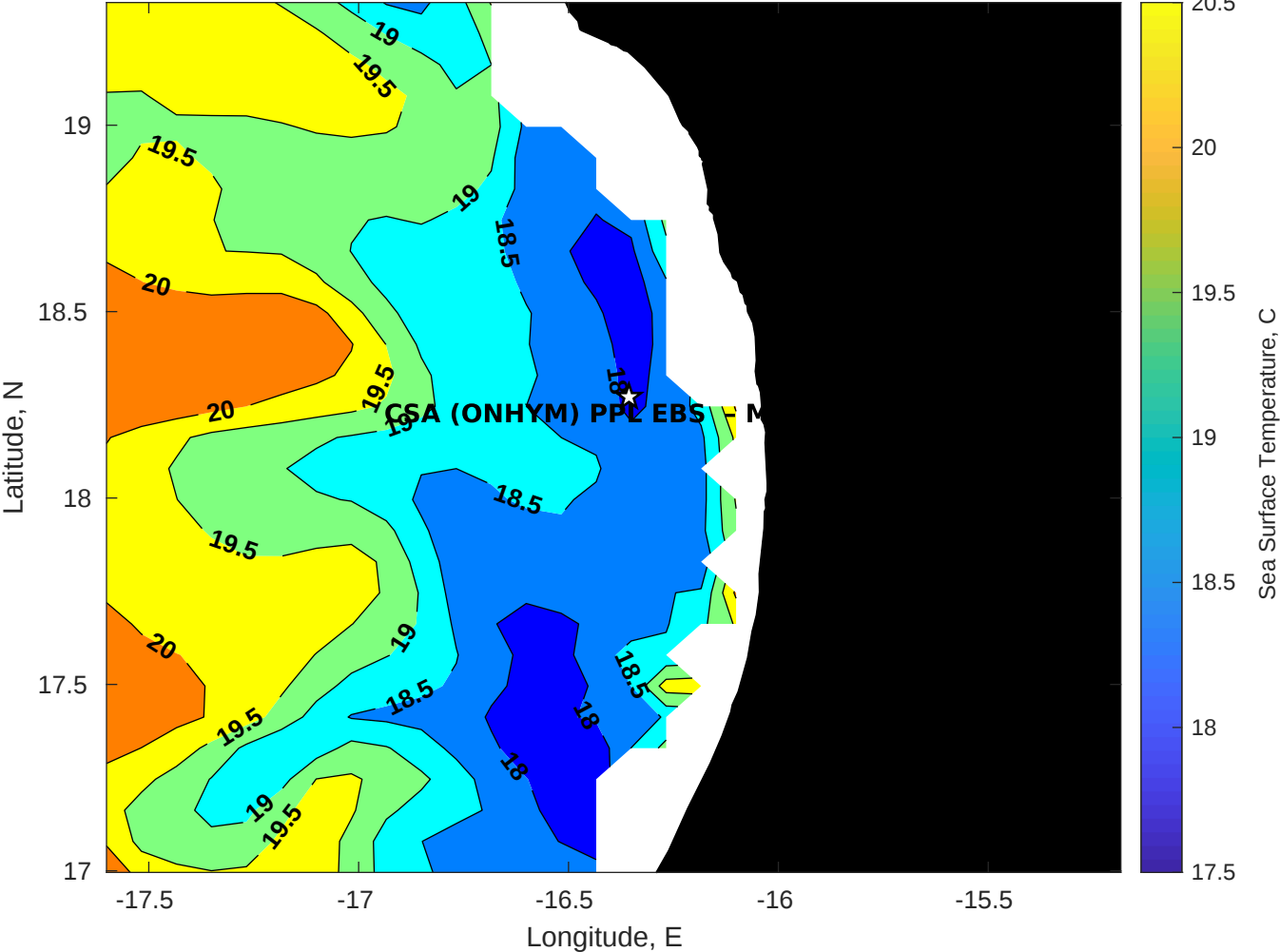
SST for CSA (ONHYM) PPL EBS - Mauritania at 27-Apr-2025 00:00:00
