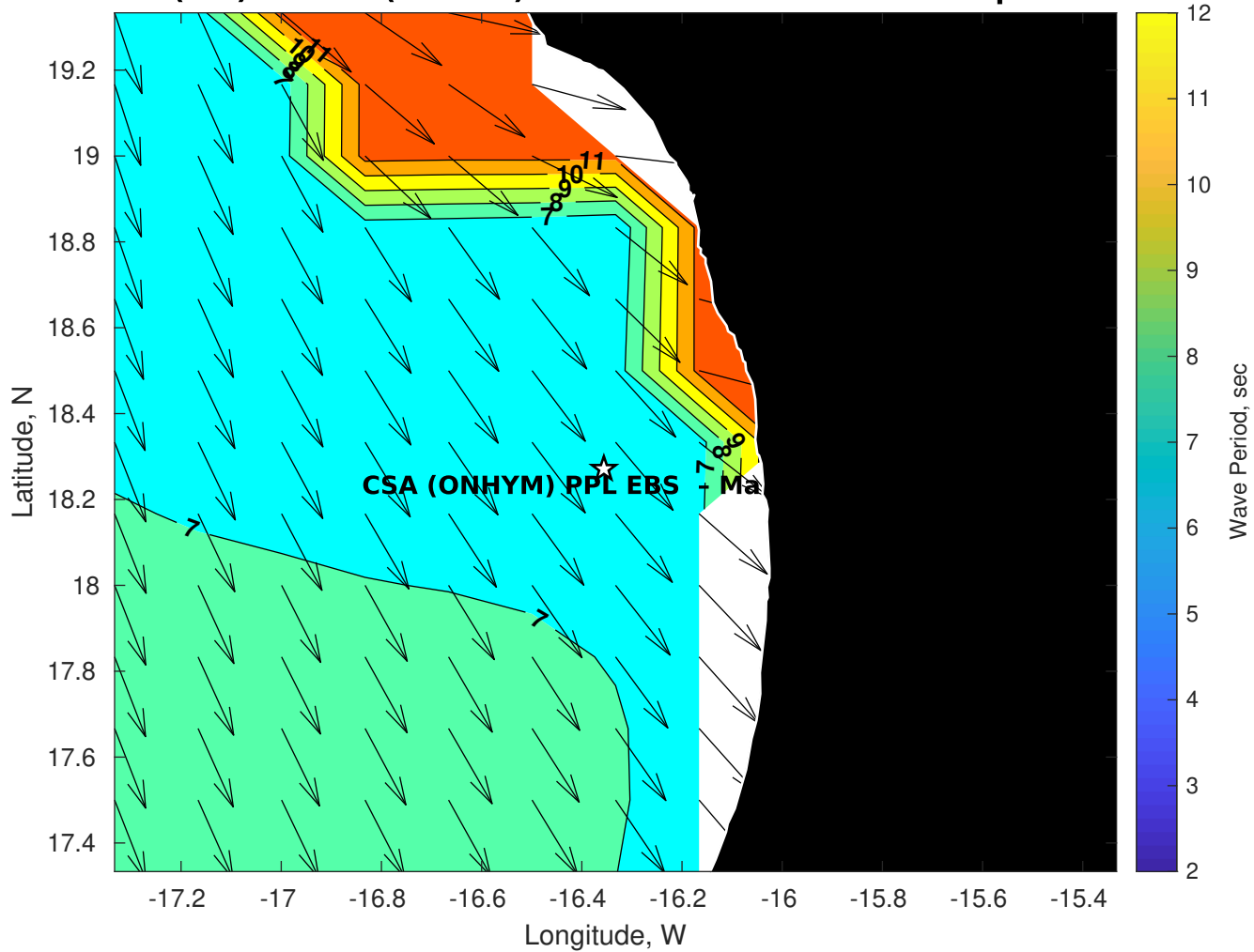
Wave Period (sec) for CSA (ONHYM) PPL EBS - Mauritania at 28-Apr-2025 09:00:00
