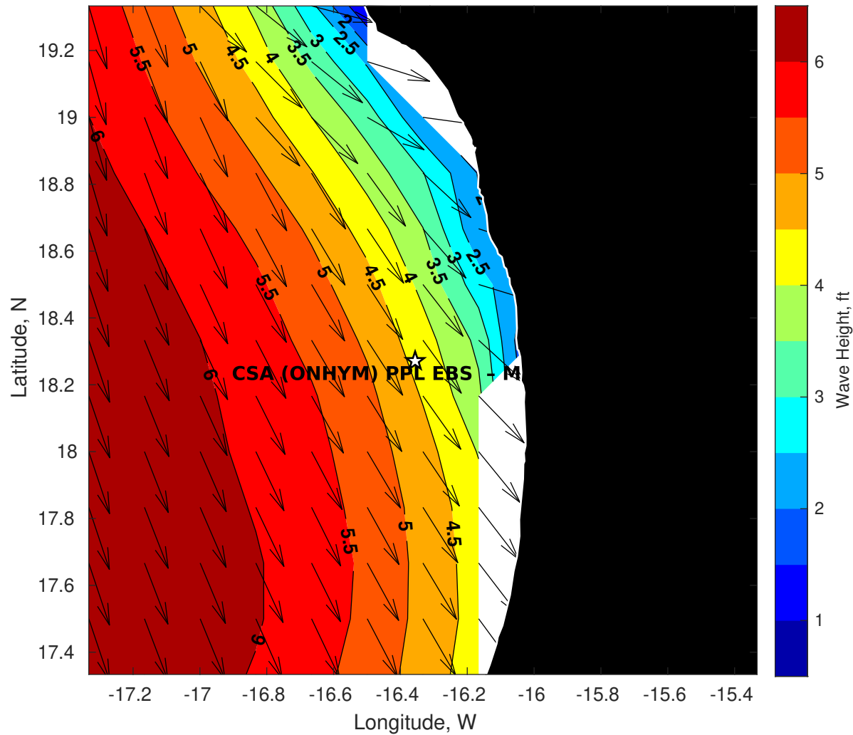
Wave Height (ft) for CSA (ONHYM) PPL EBS - Mauritania at 28-Apr-2025 09:00:00
