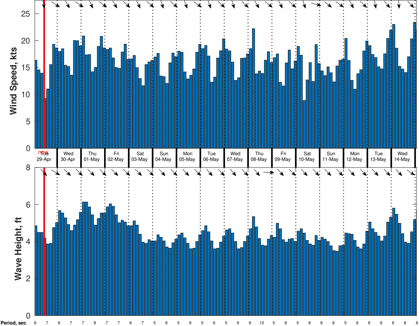
Wind & Wave Forecast for CSA (ONHYM) PPL EBS - Mauritania from 28-Apr-2025 01:00:00 to 14-May-2025 01:00:00
