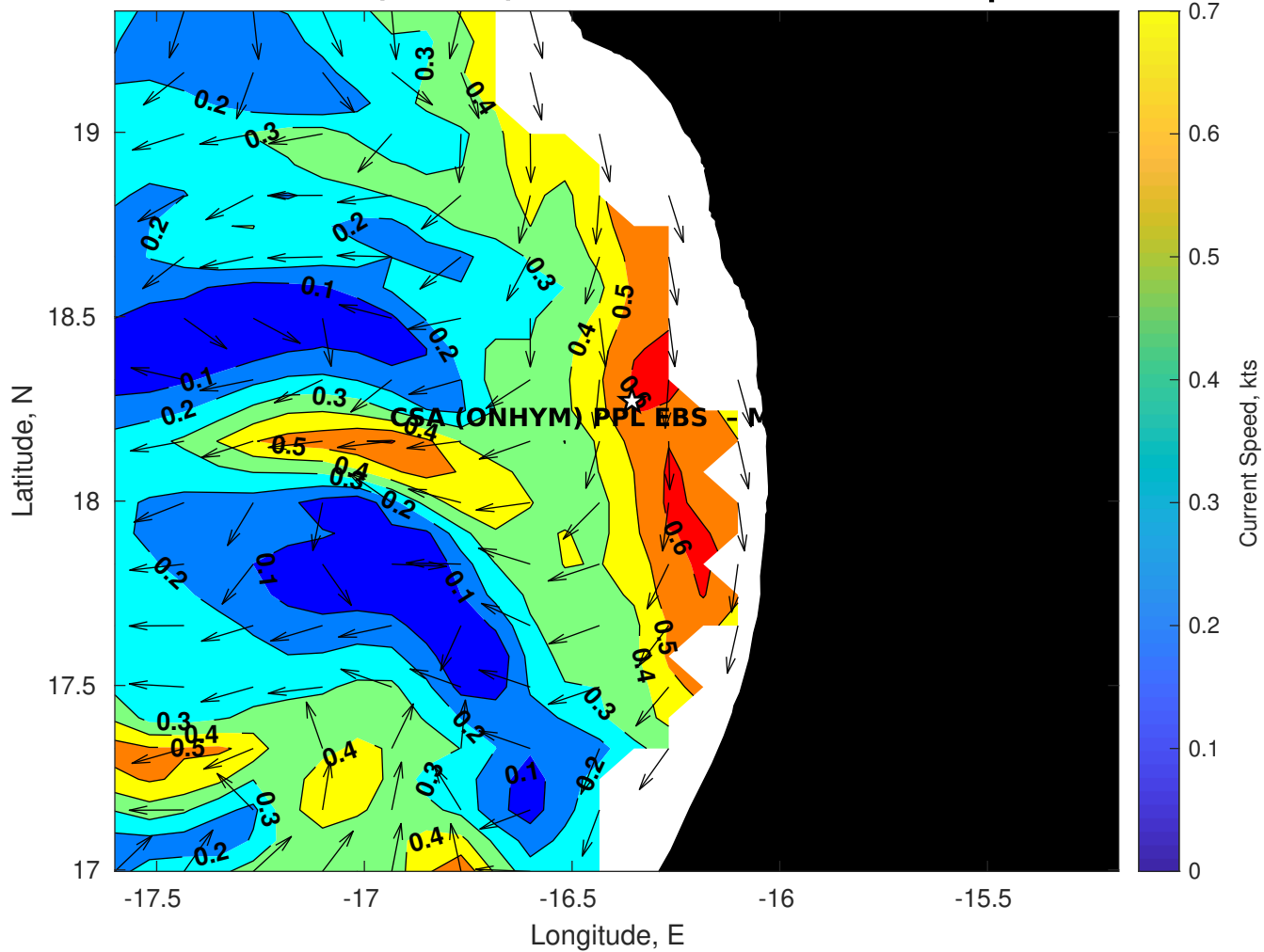
Surface Currents for CSA (ONHYM) PPL EBS - Mauritania at 27-Apr-2025 00:00:00
