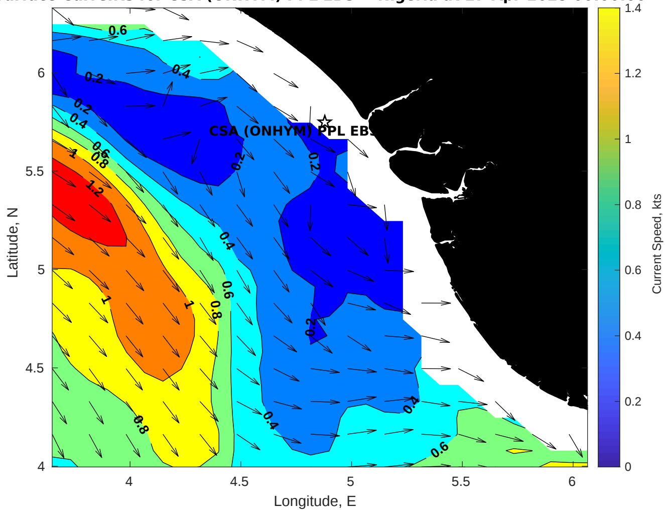
Surface Currents for CSA (ONHYM) PPL EBS - Nigeria at 27-Apr-2025 00:00:00
