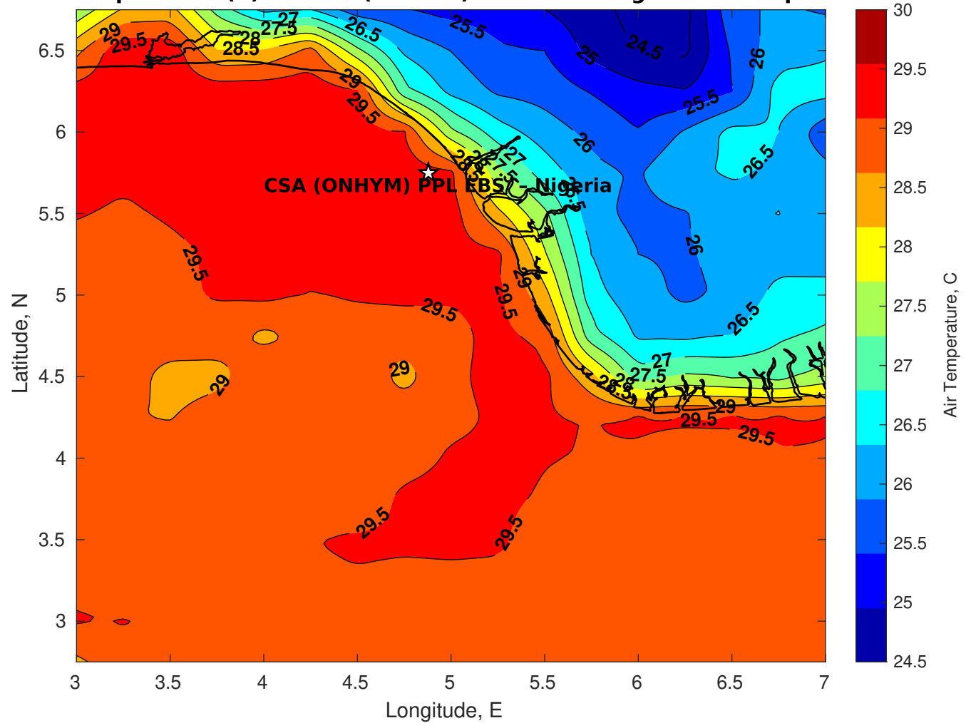
Air Temperature (C) for CSA (ONHYM) PPL EBS - Nigeria at 28-Apr-2025
