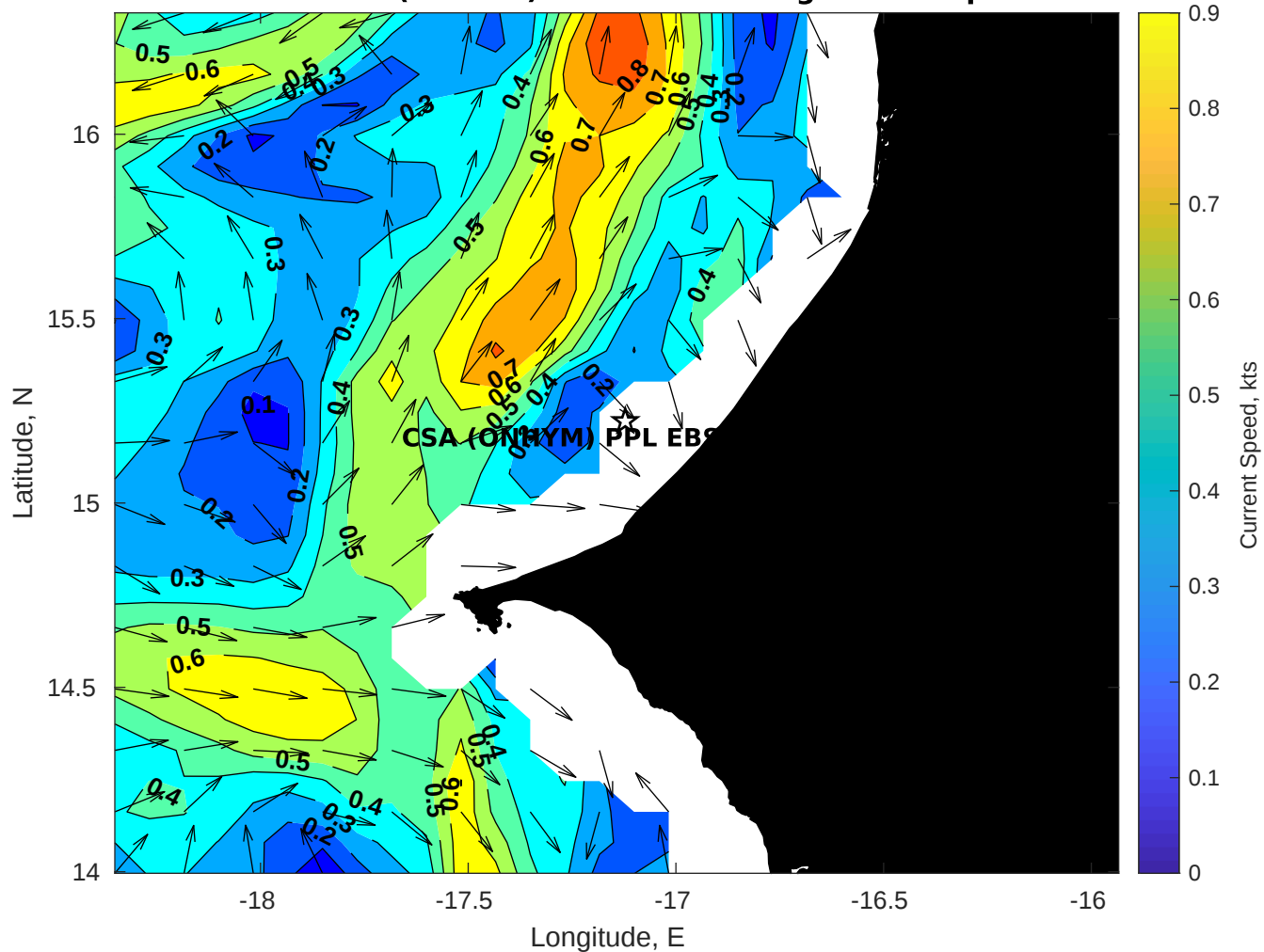
Surface Currents for CSA (ONHYM) PPL EBS - Senegal at 27-Apr-2025 00:00:00
