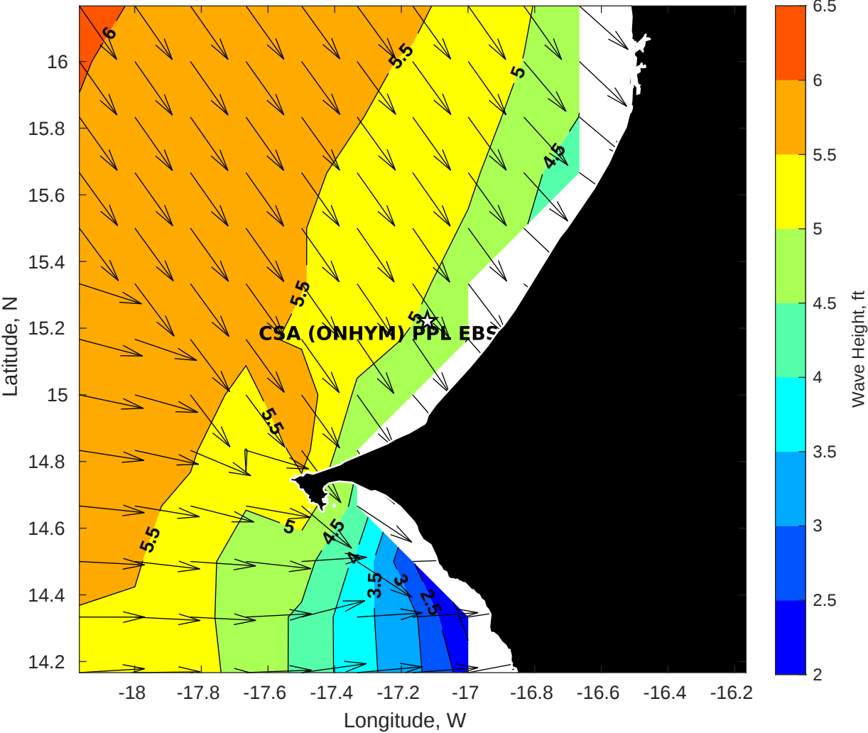
Wave Height (ft) for CSA (ONHYM) PPL EBS - Senegal at 28-Apr-2025 09:00:00
