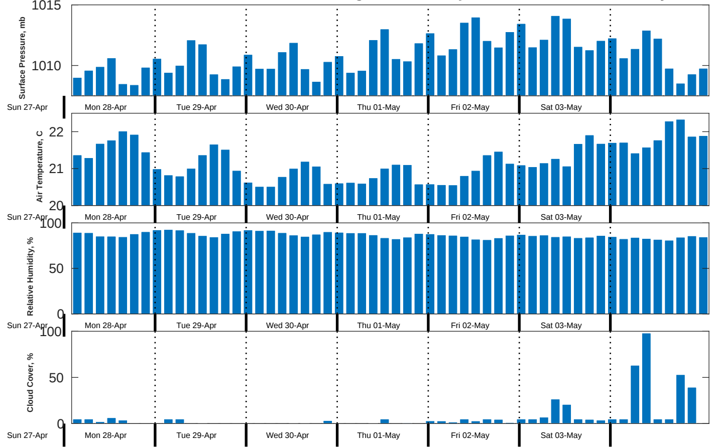
Met Forecast for CSA (ONHYM) PPL EBS - Senegal from 28-Apr-2025 00:00:00 to 05-May-2025 00:00:00
