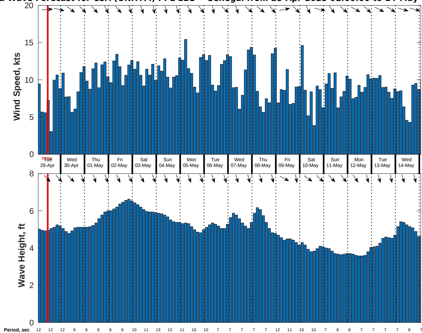
Wind & Wave Forecast for CSA (ONHYM) PPL EBS - Senegal from 28-Apr-2025 01:00:00 to 14-May-2025 01:00:00
