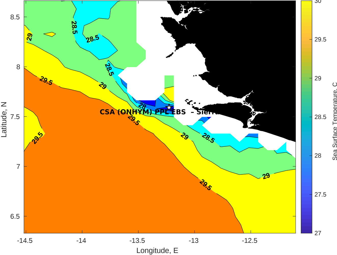
SST for CSA (ONHYM) PPL EBS - Sierra Leone at 27-Apr-2025 00:00:00
