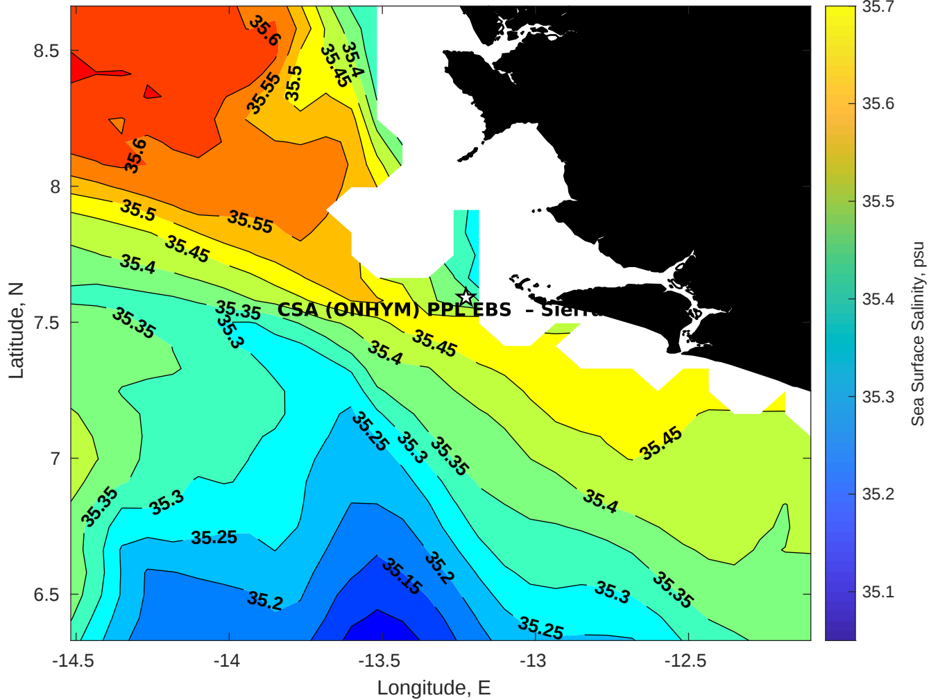
Surface Salinity for CSA (ONHYM) PPL EBS - Sierra Leone at 27-Apr-2025 00:00:00
