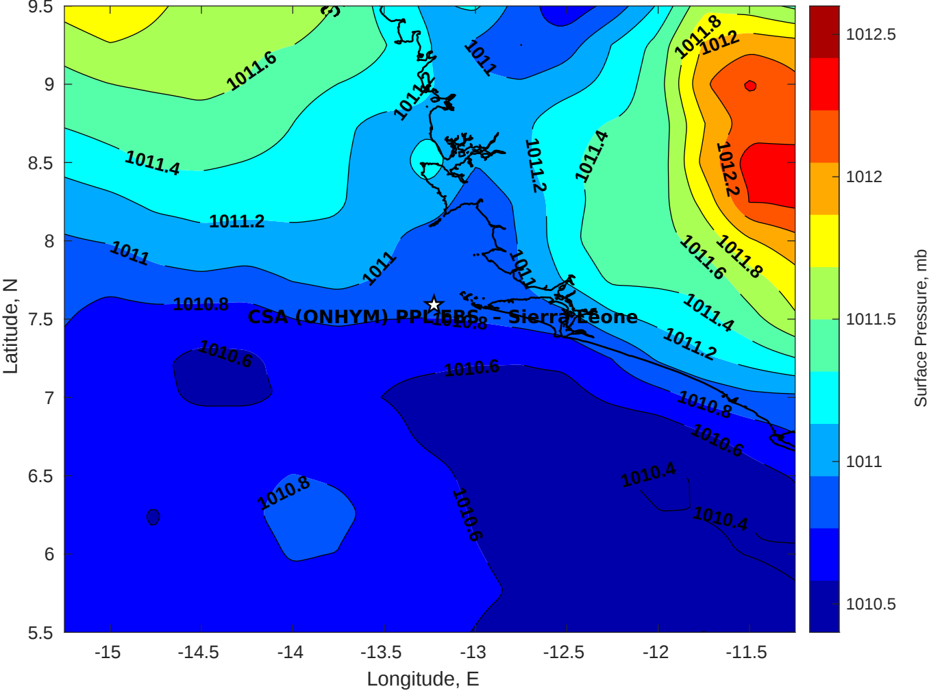
Surface Pressure (mb) for CSA (ONHYM) PPL EBS - Sierra Leone at 28-Apr-2025 00:00:00
