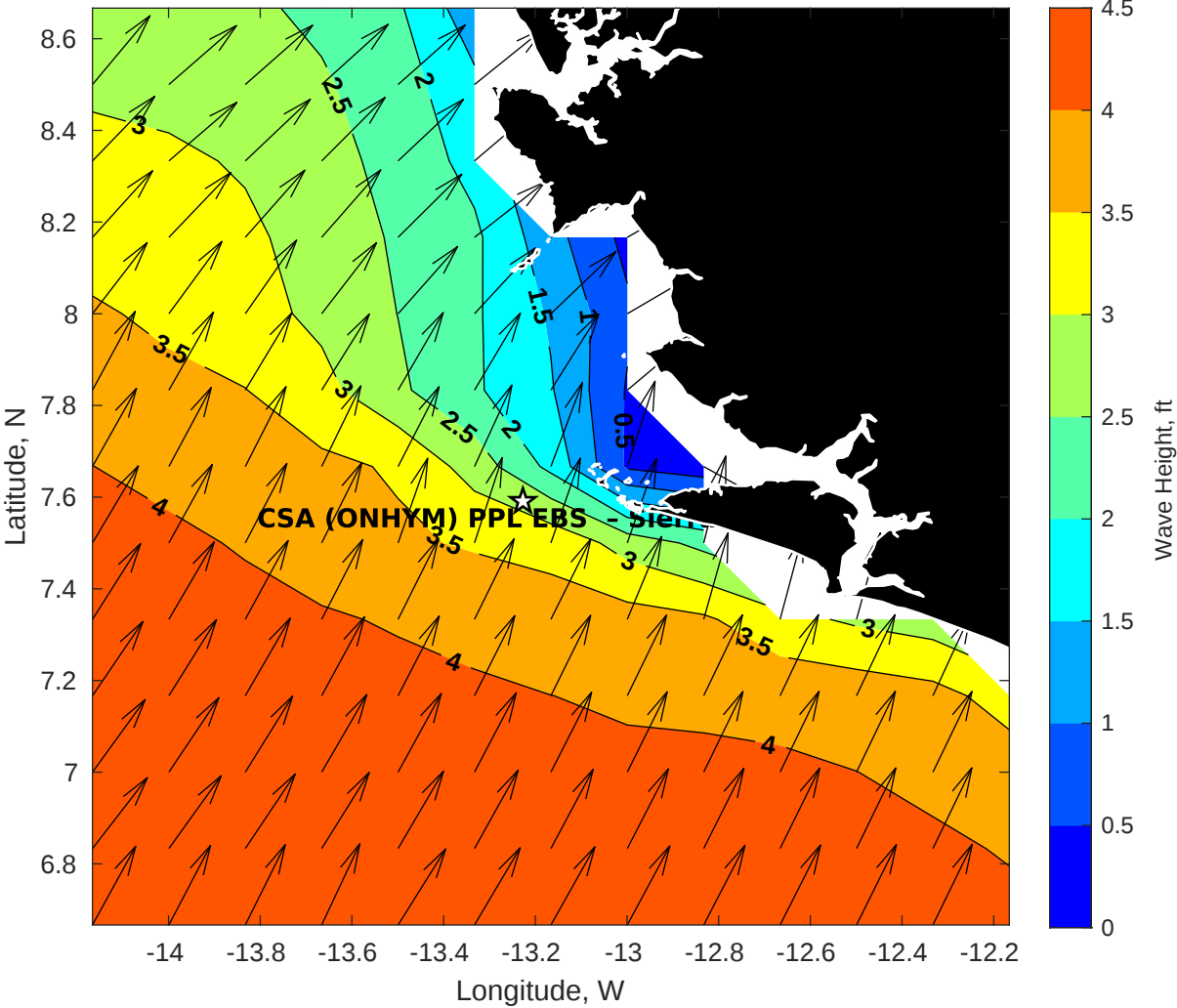
Wave Height (ft) for CSA (ONHYM) PPL EBS - Sierra Leone at 28-Apr-2025 09:00:00
