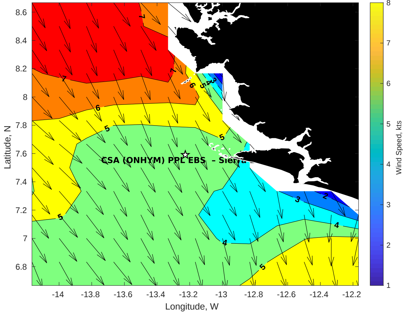
Winds (kts) for CSA (ONHYM) PPL EBS - Sierra Leone at 28-Apr-2025 09:00:00
