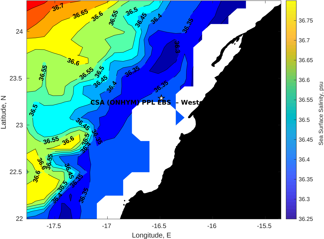
Surface Salinity for CSA (ONHYM) PPL EBS - Western Sahara at 27-Apr-2025 00:00:00
