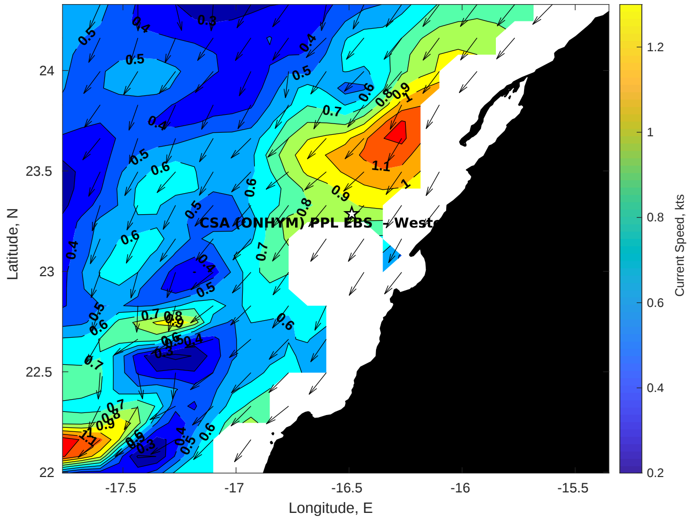
Surface Currents for CSA (ONHYM) PPL EBS - Western Sahara at 27-Apr-2025 00:00:00
