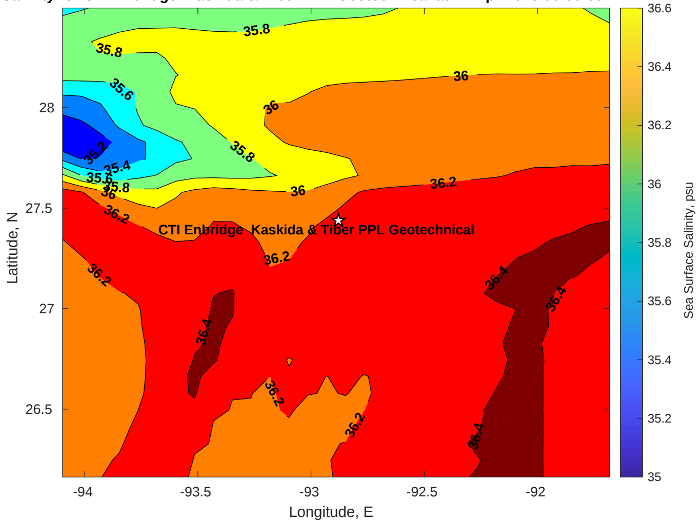
Surface Salinity for CTI Enbridge Kaskida & Tiber PPL Geotechnical at 27-Apr-2025 00:00:00
