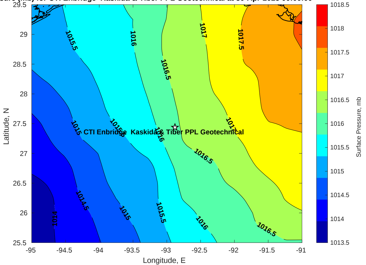
Surface Pressure (mb) for CTI Enbridge Kaskida & Tiber PPL Geotechnical at 30-Apr-2025 00:00:00
