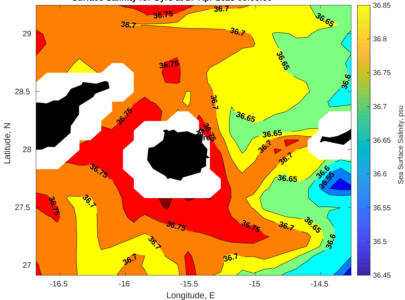
Surface Salinity for Gyre at 27-Apr-2025 00:00:00
