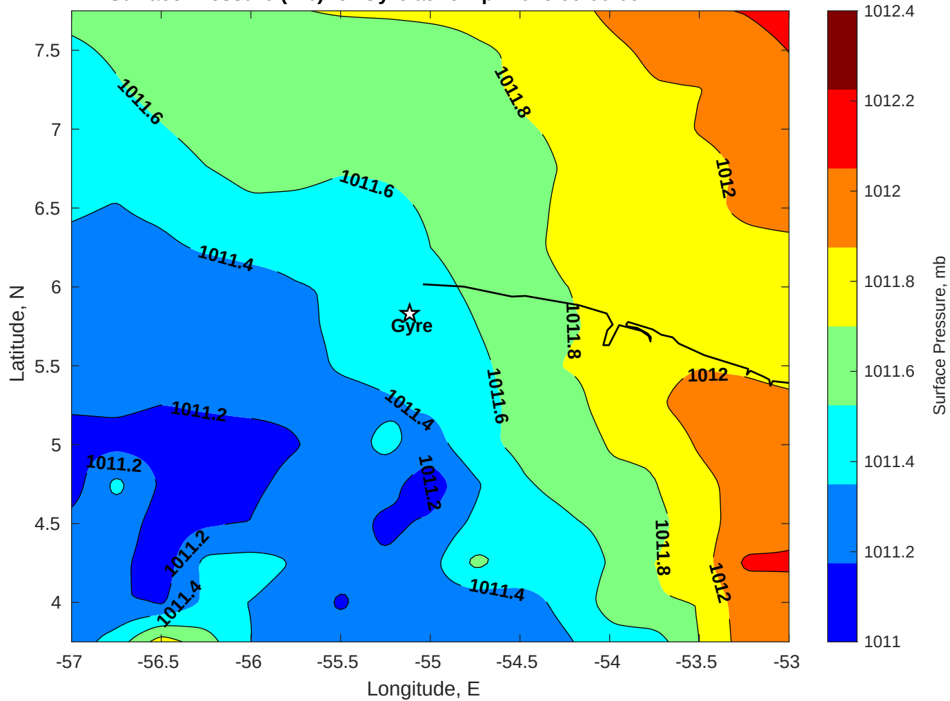
Surface Pressure (mb) for Gyre at 29-Apr-2025 00:00:00
