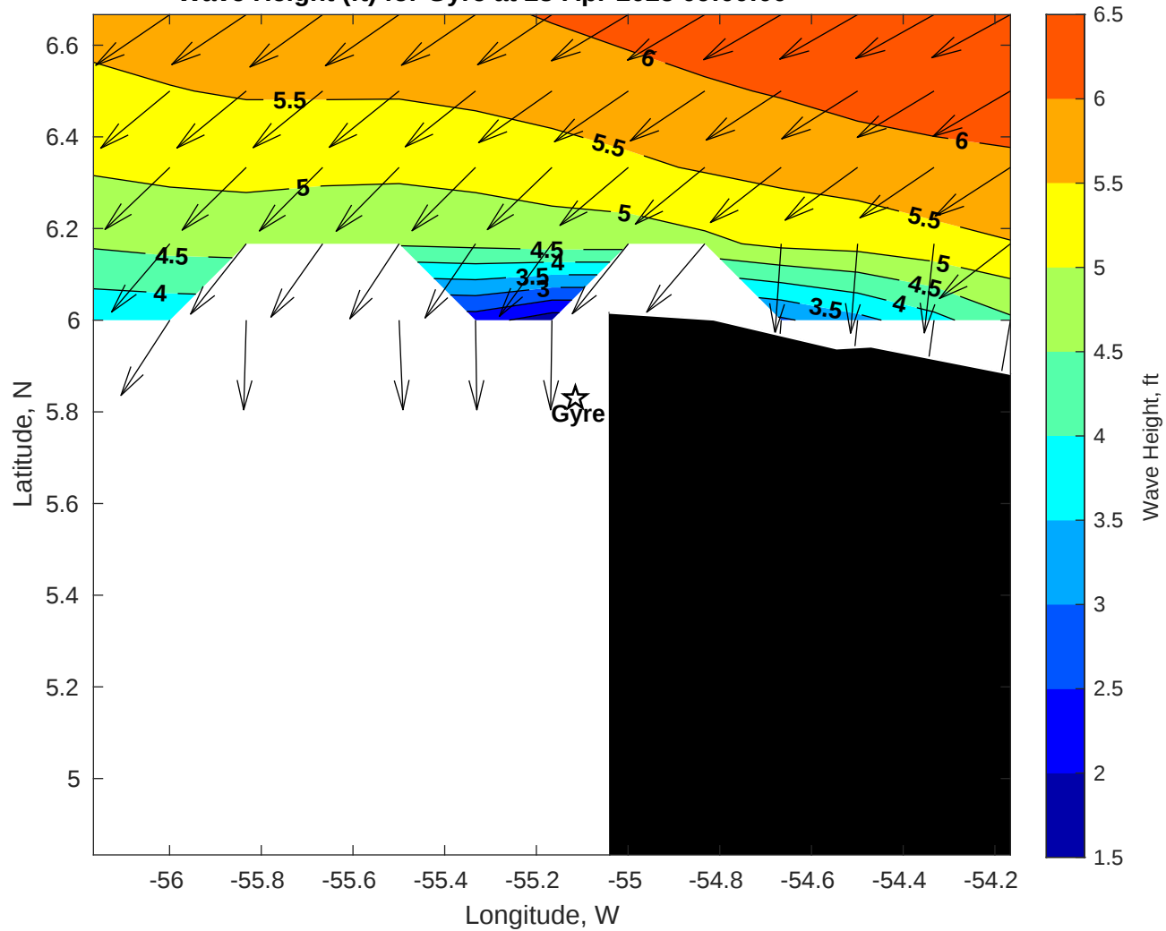
Wave Height (ft) for Gyre at 28-Apr-2025 09:00:00
