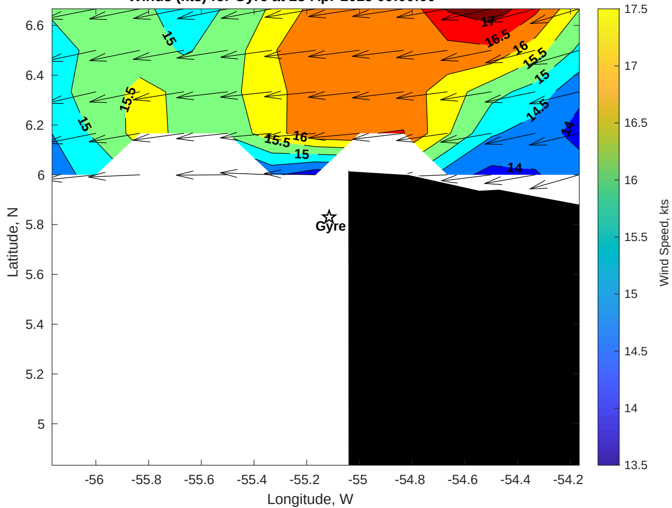
Winds (kts) for Gyre at 28-Apr-2025 09:00:00
