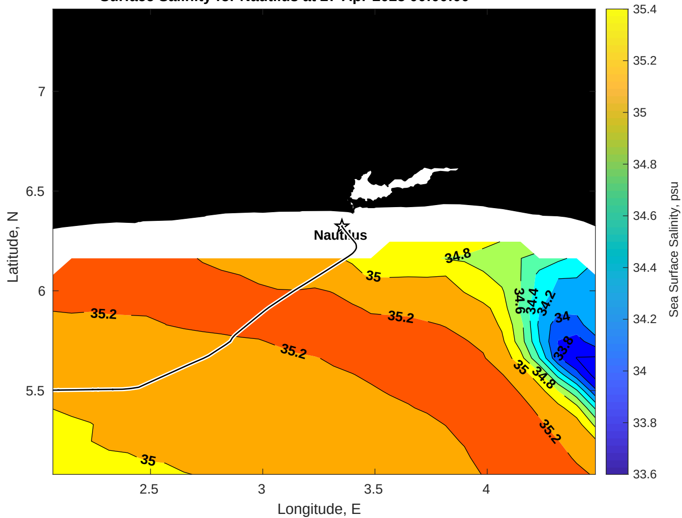
Surface Salinity for Nautilus at 27-Apr-2025 00:00:00
