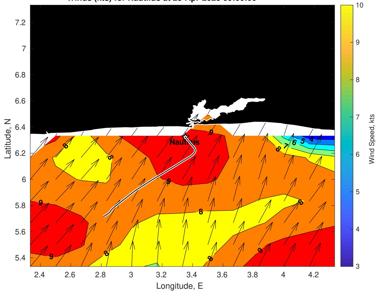
Winds (kts) for Nautilus at 28-Apr-2025 09:00:00
