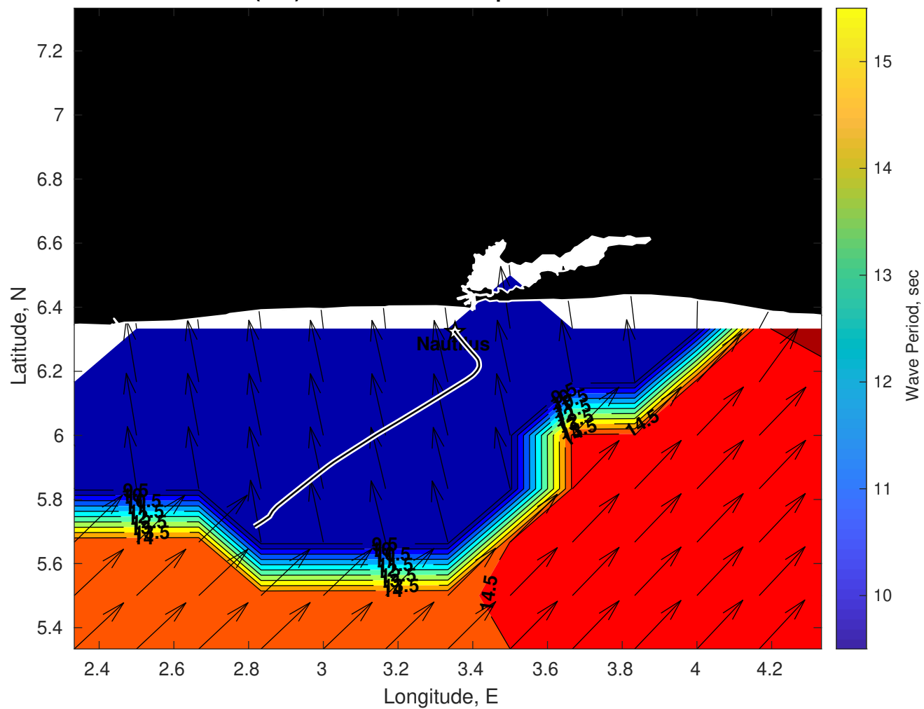
Wave Period (sec) for Nautilus at 28-Apr-2025 09:00:00
