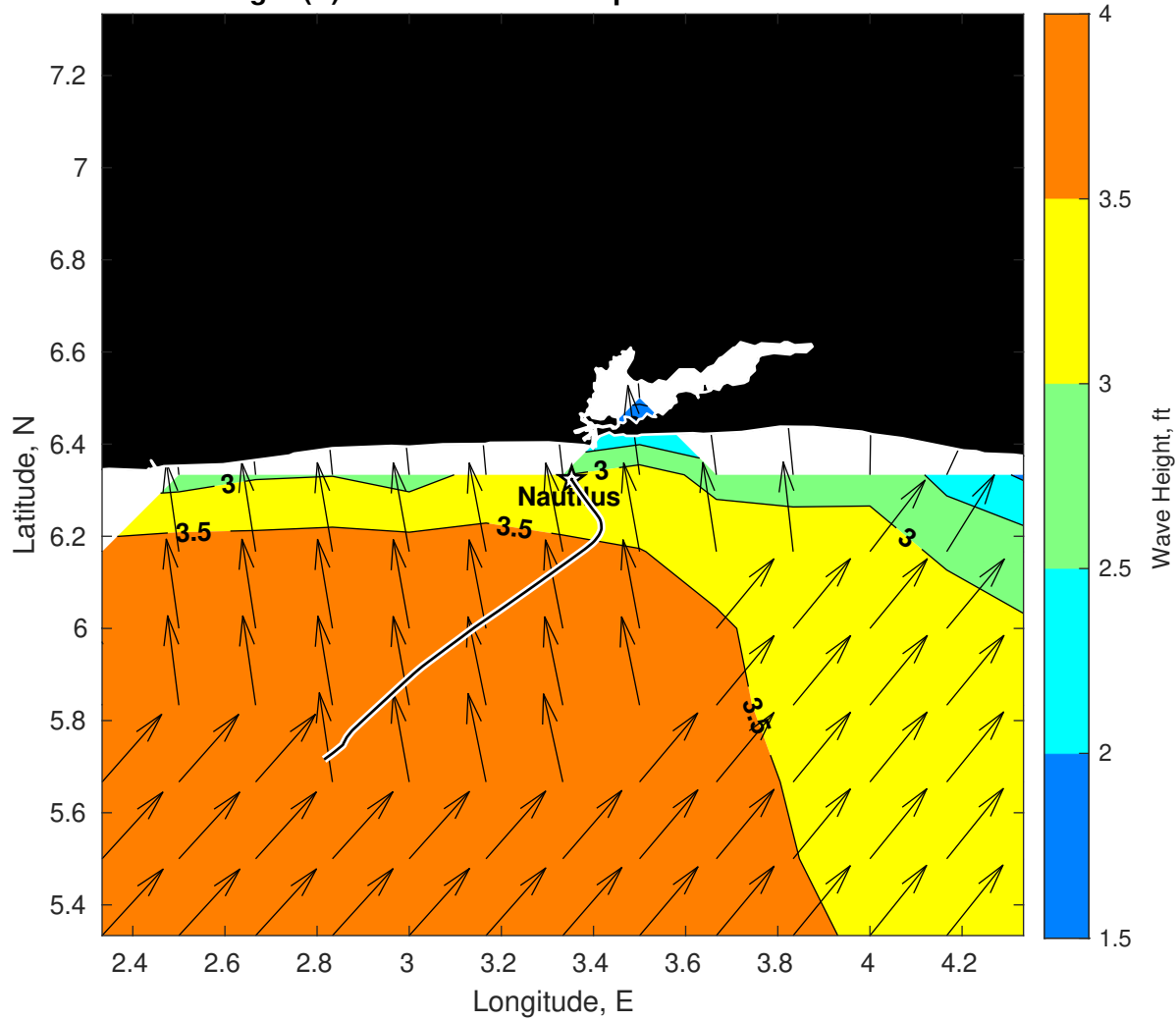
Wave Height (ft) for Nautilus at 28-Apr-2025 09:00:00
