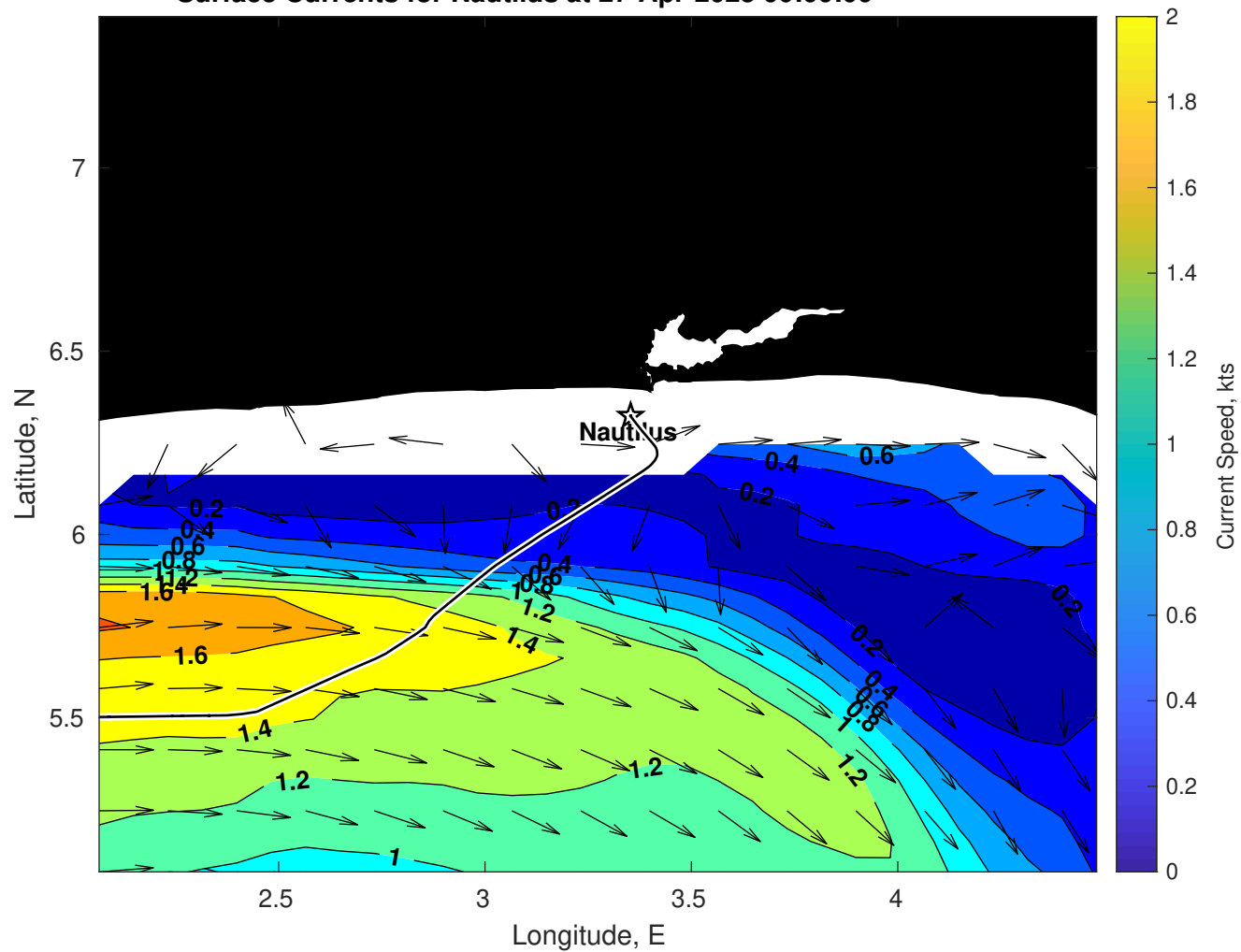
Surface Currents for Nautilus at 27-Apr-2025 00:00:00
