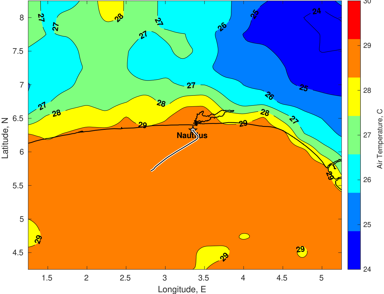
Air Temperature (C) for Nautilus at 28-Apr-2025
