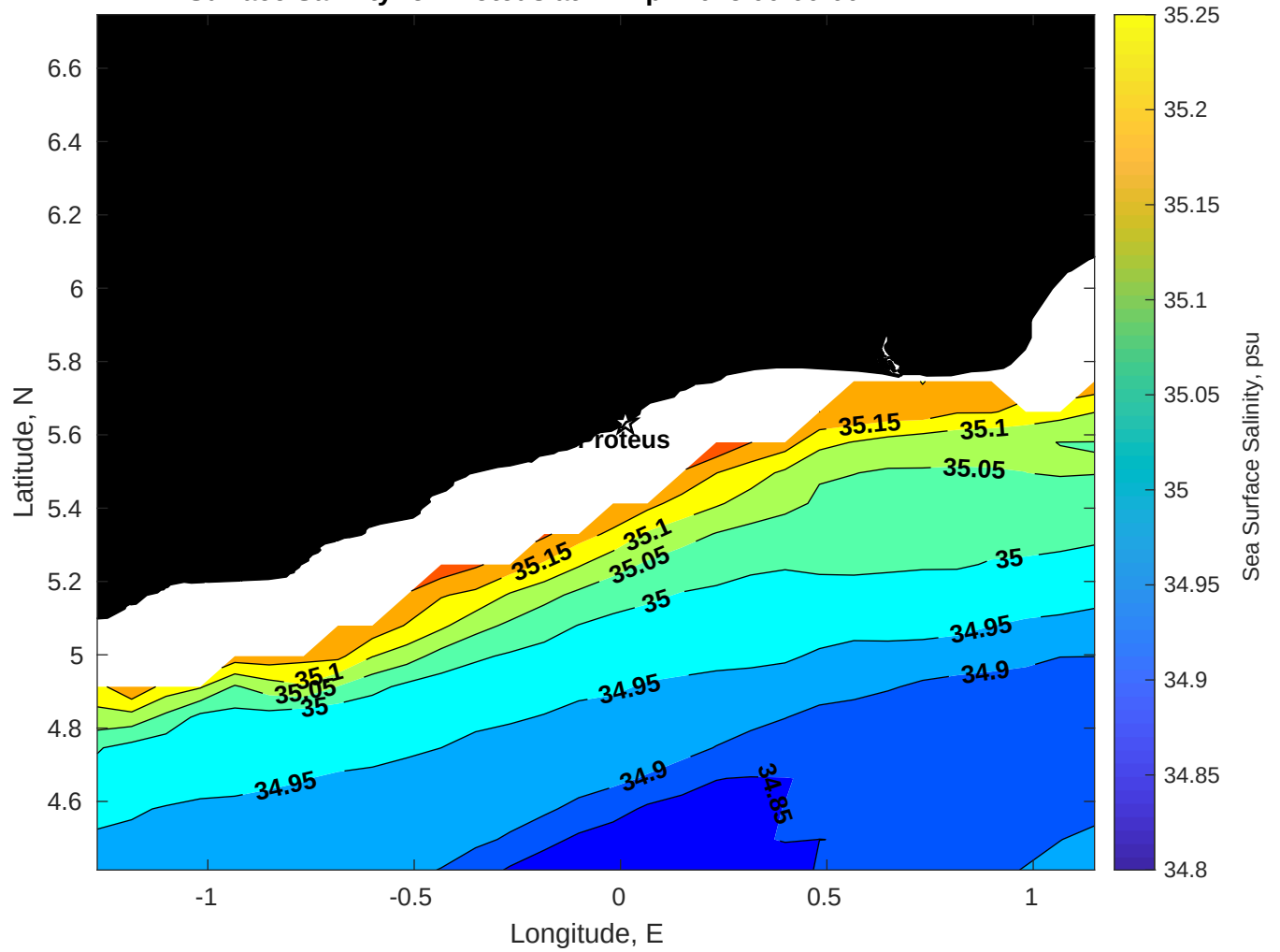
Surface Salinity for Proteus at 27-Apr-2025 00:00:00
