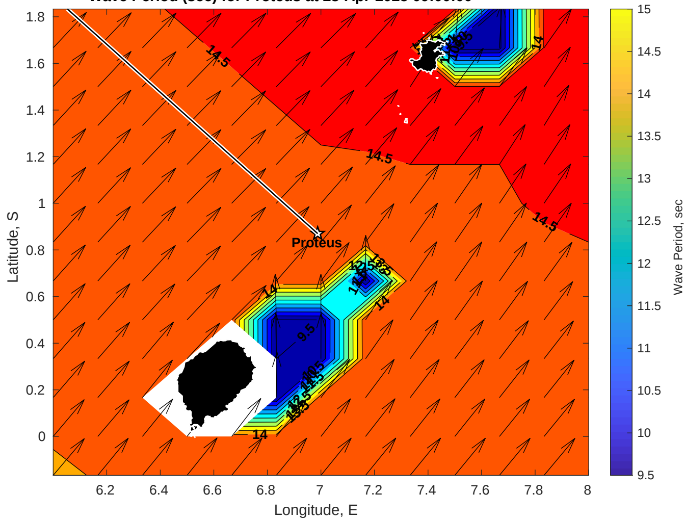
Wave Period (sec) for Proteus at 28-Apr-2025 09:00:00
