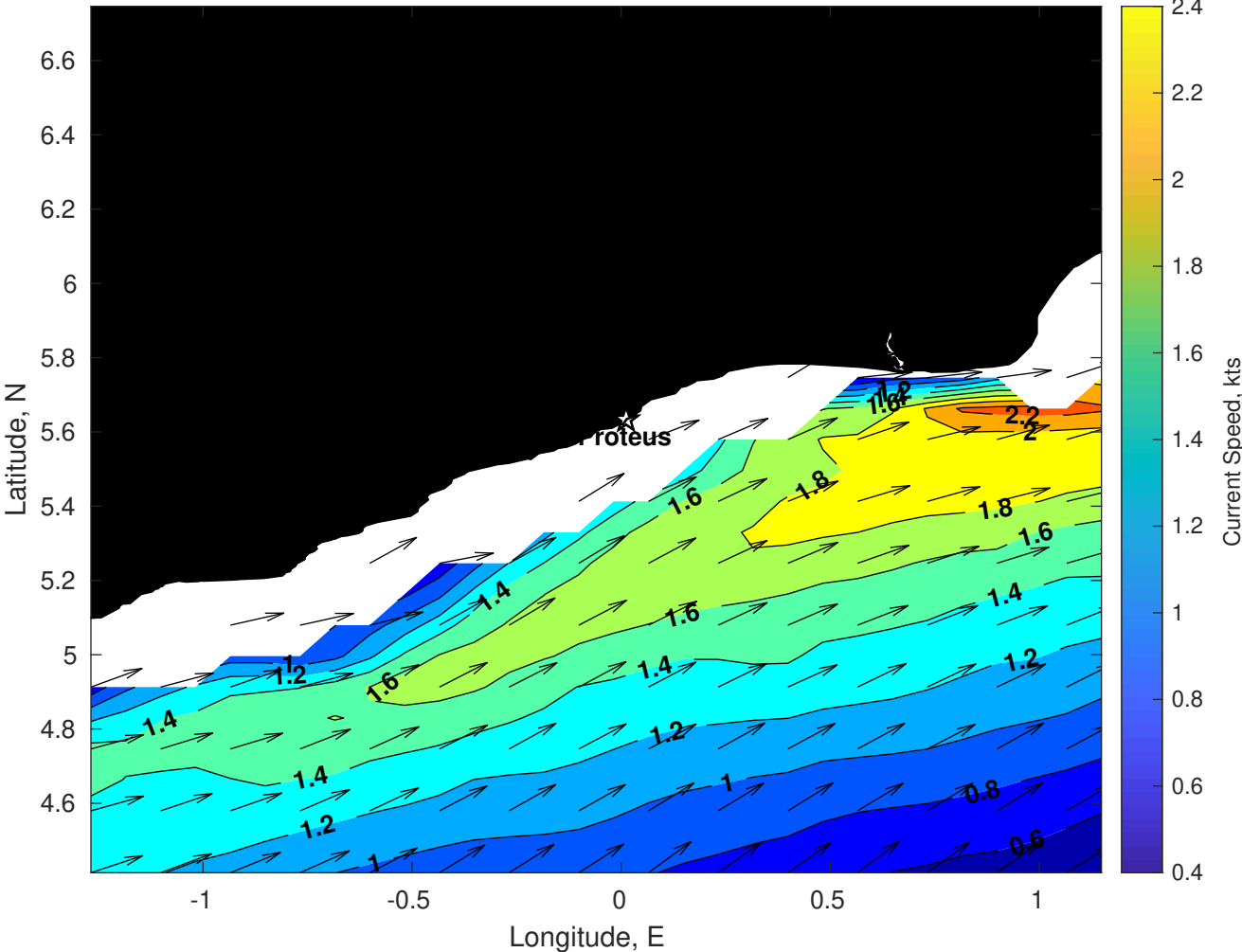
Surface Currents for Proteus at 27-Apr-2025 00:00:00
