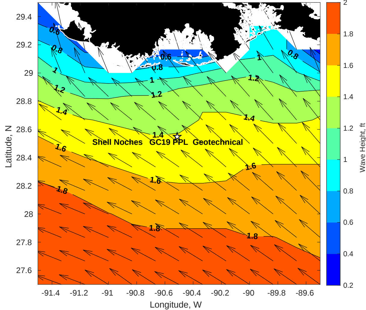
Wave Height (ft) for Shell Noches GC19 PPL Geotechnical at 28-Apr-2025 09:00:00
