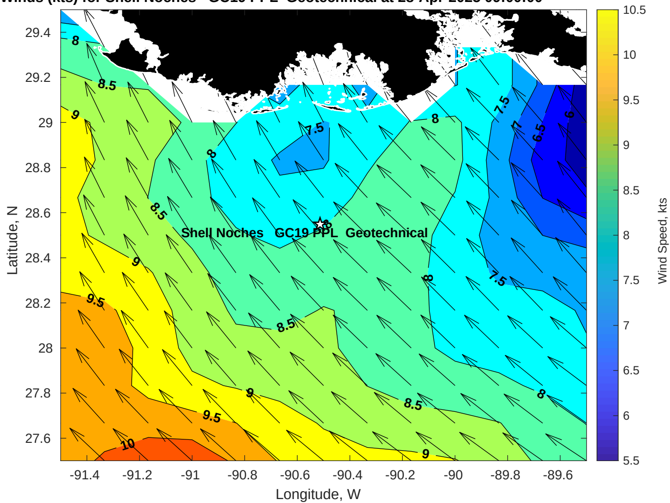
Winds (kts) for Shell Noches GC19 PPL Geotechnical at 28-Apr-2025 09:00:00
