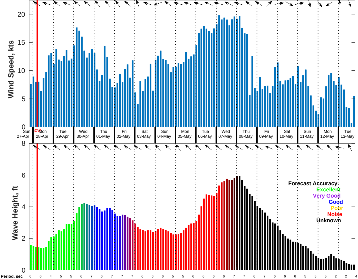
Wind & Wave Forecast for Shell Noches GC19 PPL Geotechnical from 27-Apr-2025 20:00:00 to 13-May-2025 20:00:00
