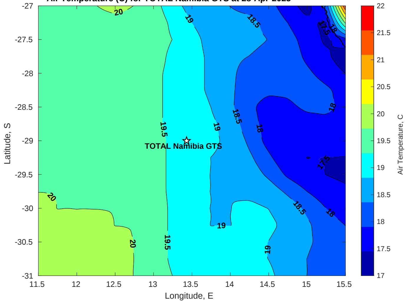
Air Temperature (C) for TOTAL Namibia GTS at 28-Apr-2025
