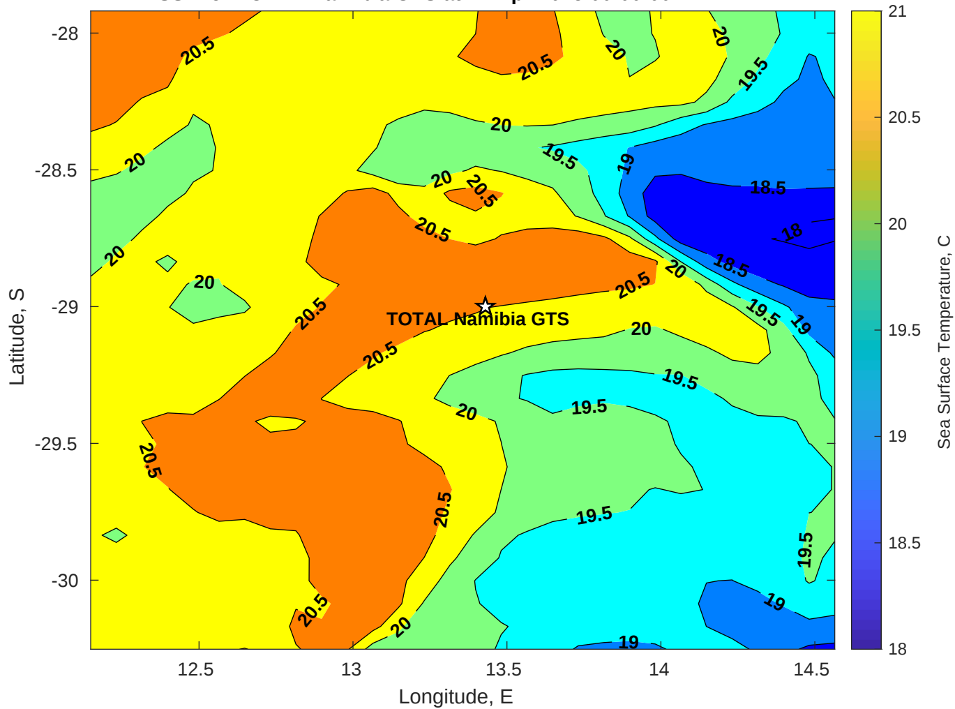
SST for TOTAL Namibia GTS at 27-Apr-2025 00:00:00
