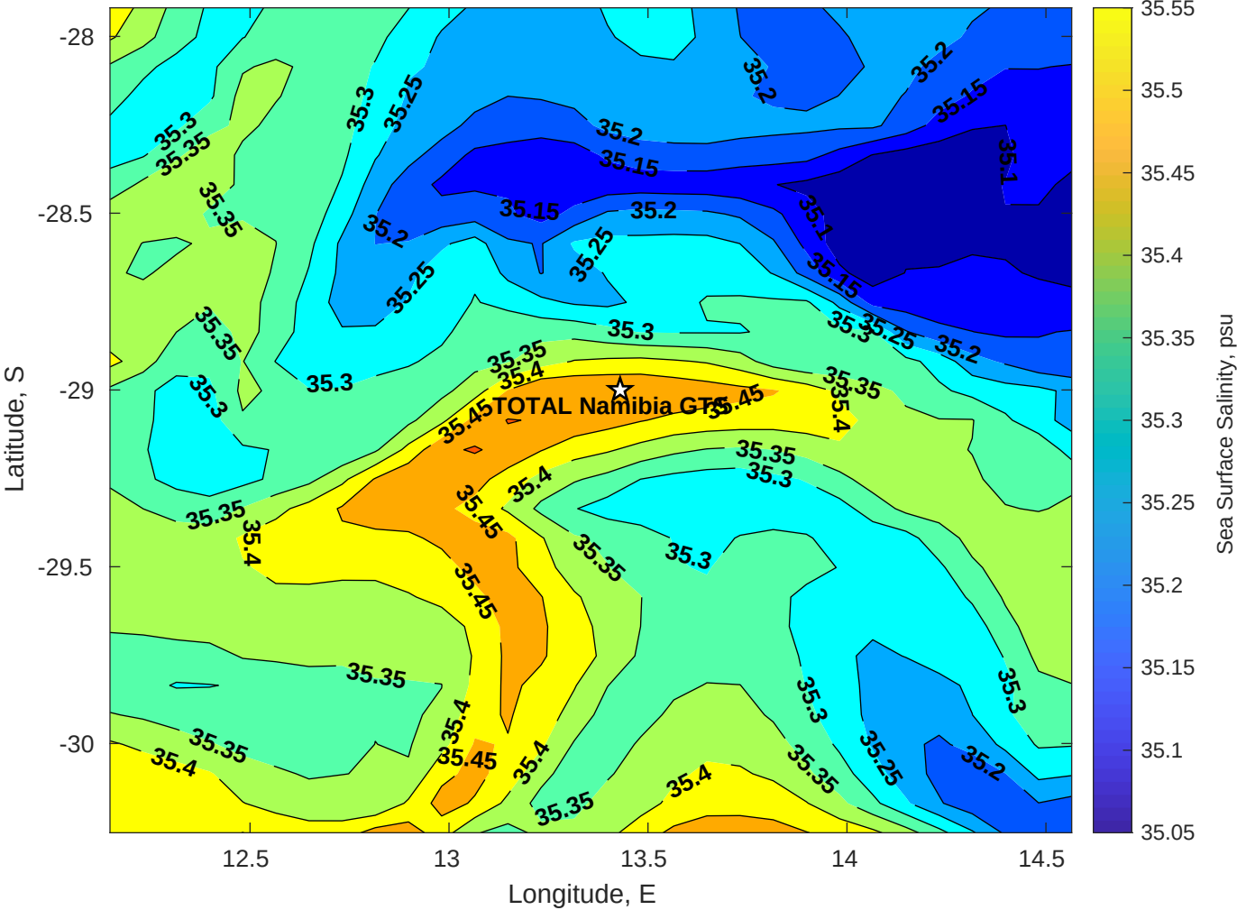
Surface Salinity for TOTAL Namibia GTS at 27-Apr-2025 00:00:00
