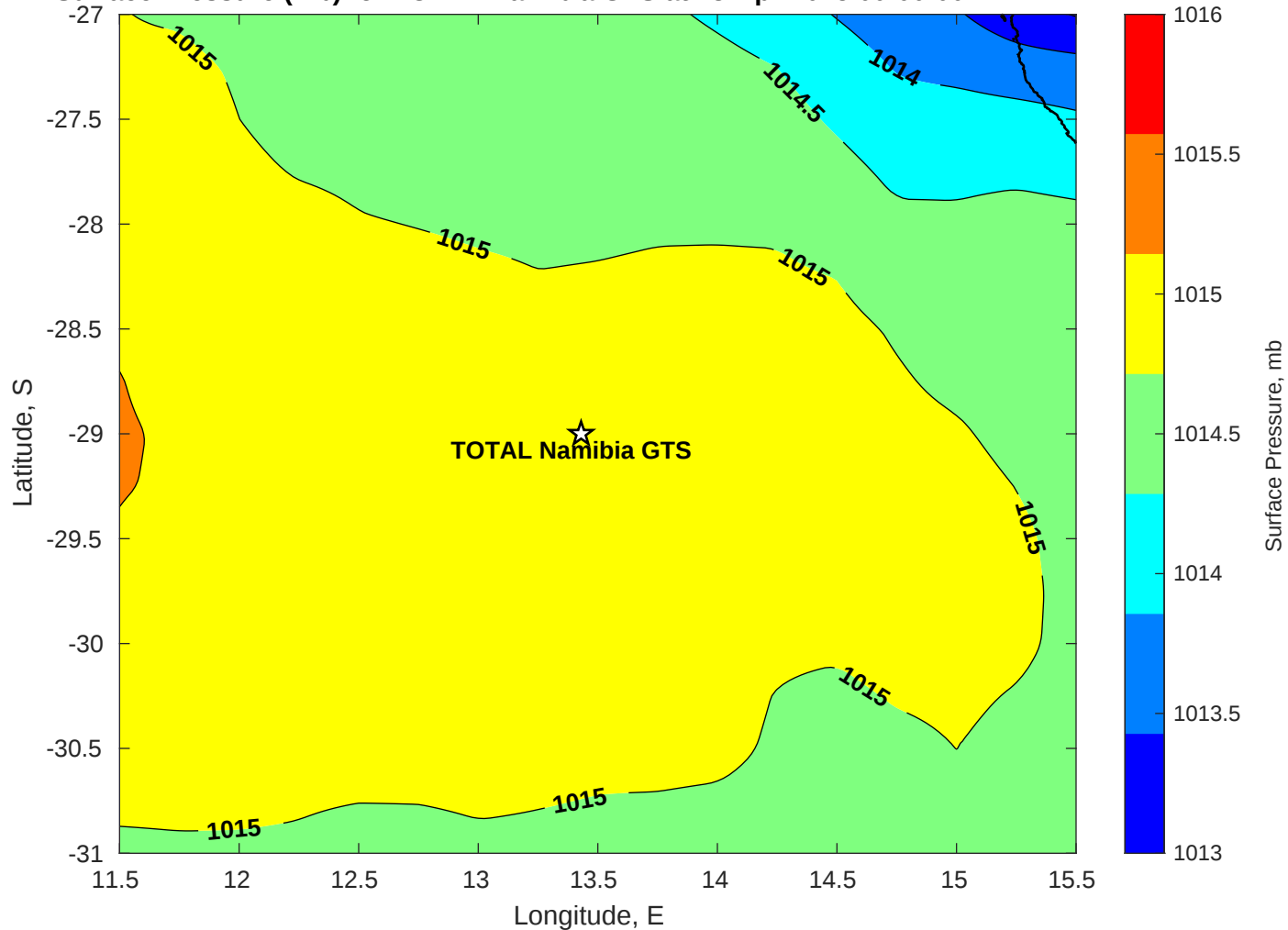
Surface Pressure (mb) for TOTAL Namibia GTS at 28-Apr-2025 00:00:00
