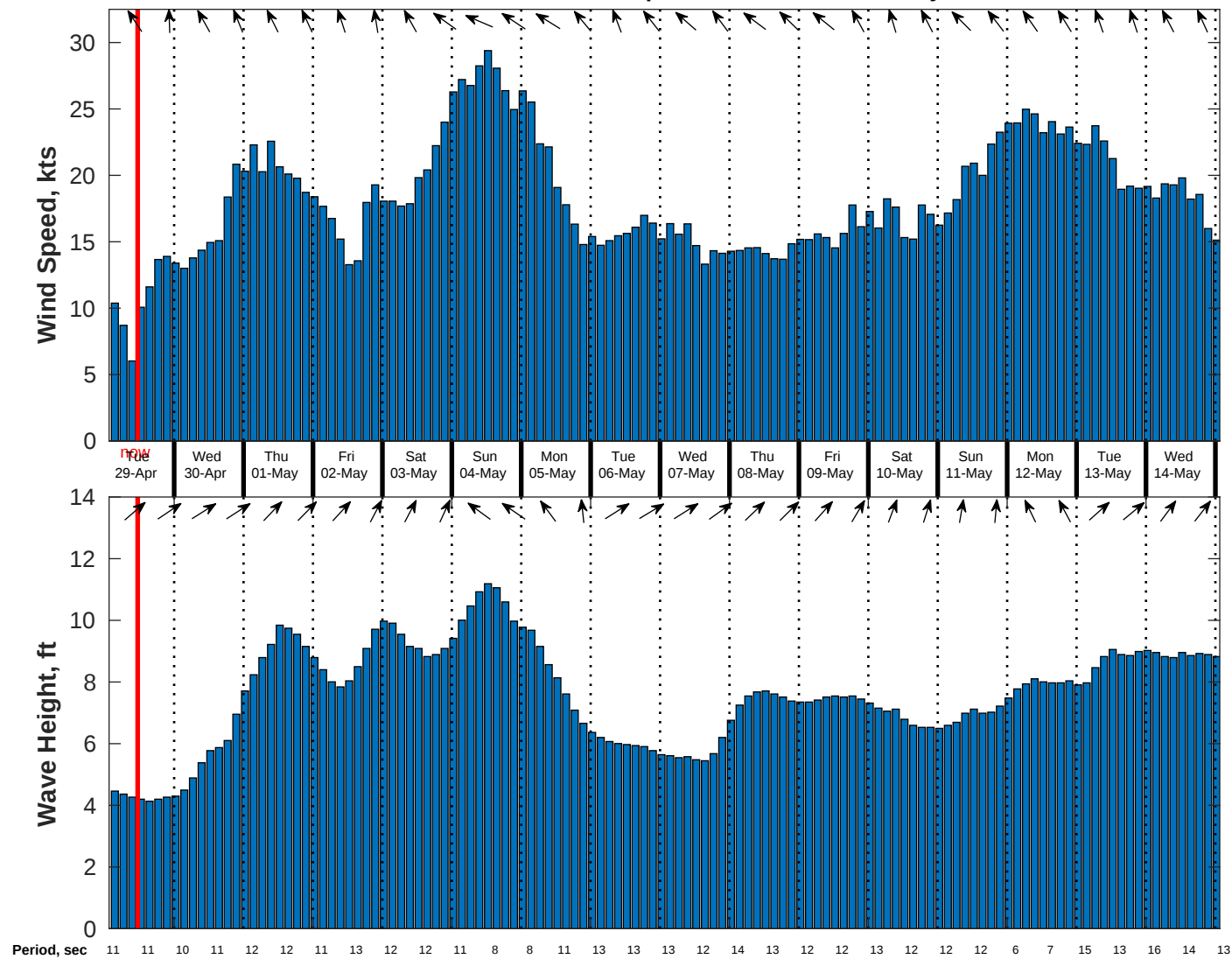
Wind & Wave Forecast for TOTAL Namibia GTS from 28-Apr-2025 02:00:00 to 14-May-2025 02:00:00
